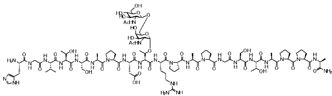
Compound 10
