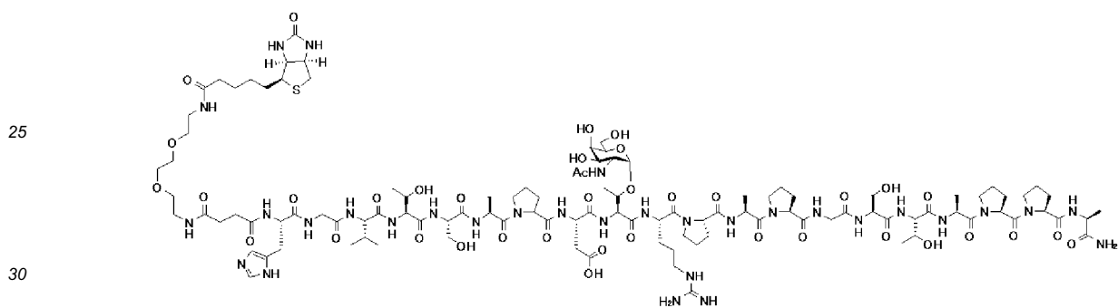
Compound 18
