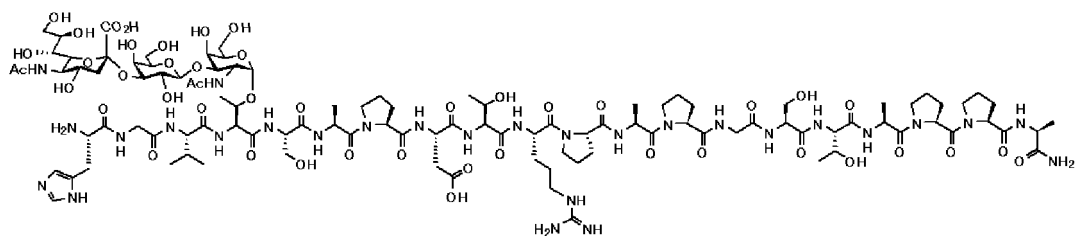
Compound 13
