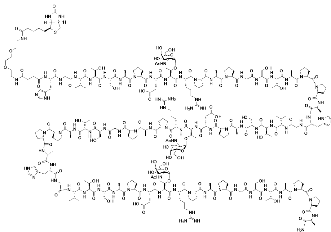
Compound 20
