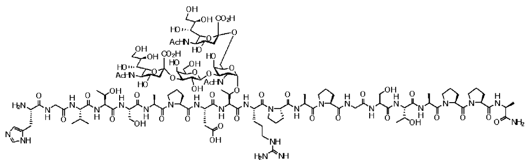
Compound 12
