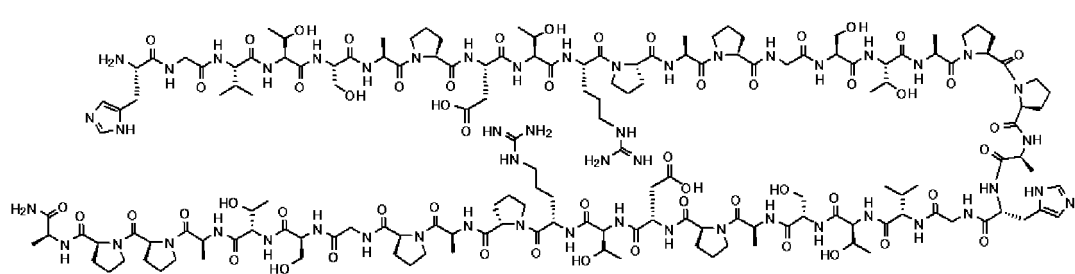
Compound 14
