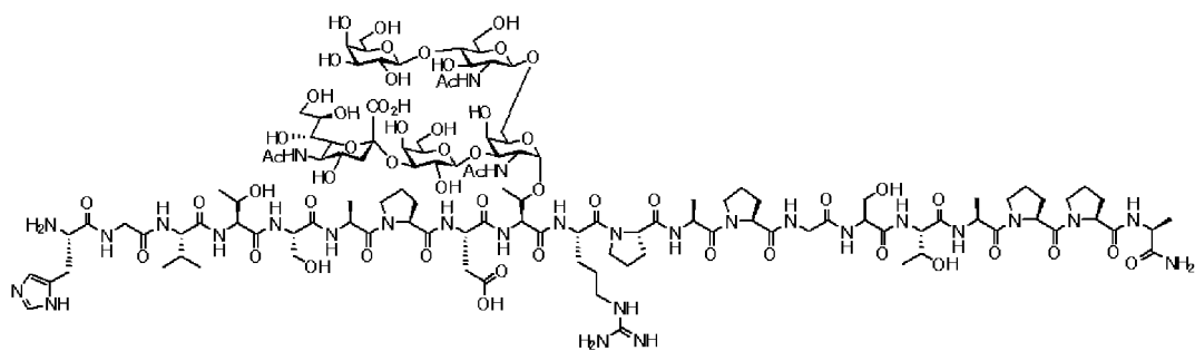
Compound 8
