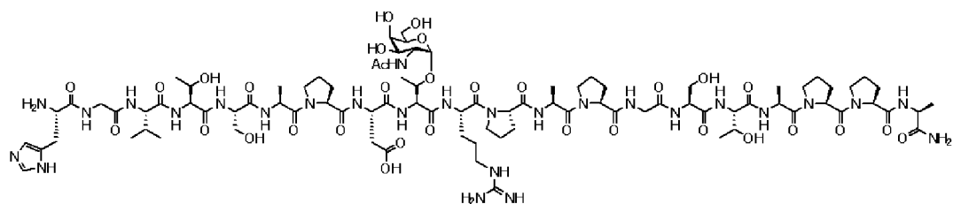
Compound 4
