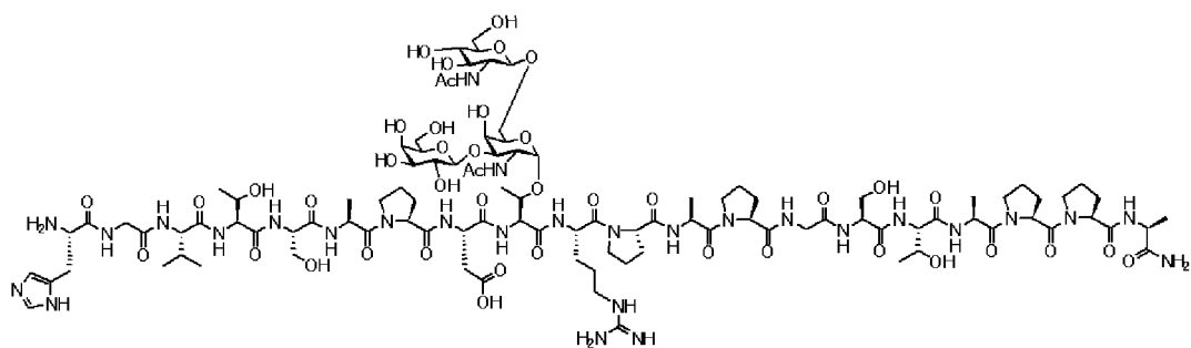
Compound 6
