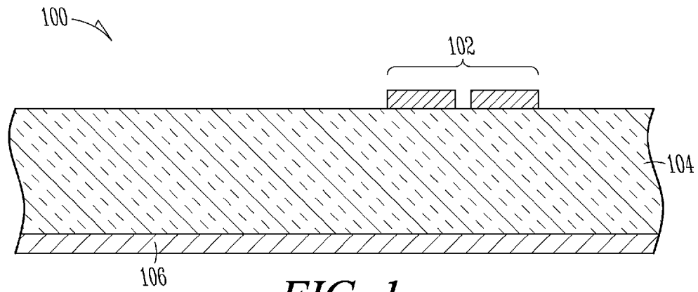
FIG. 1 (PRIOR ART)
