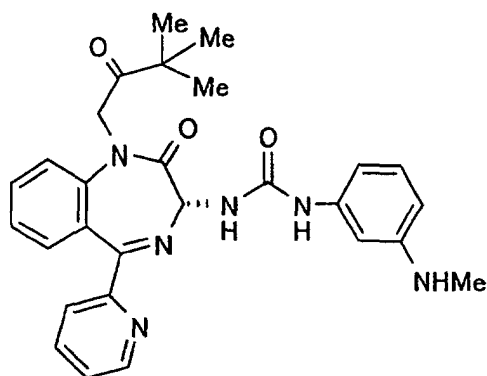
Compound A
