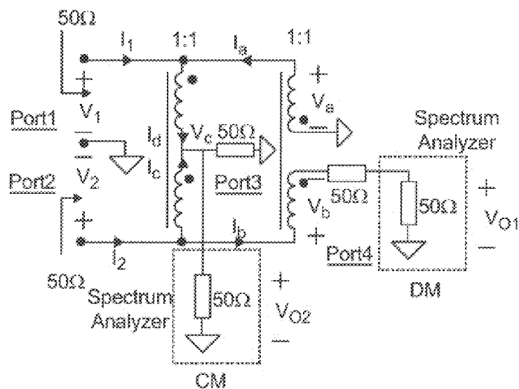
Figure 2 PRIOR ART
