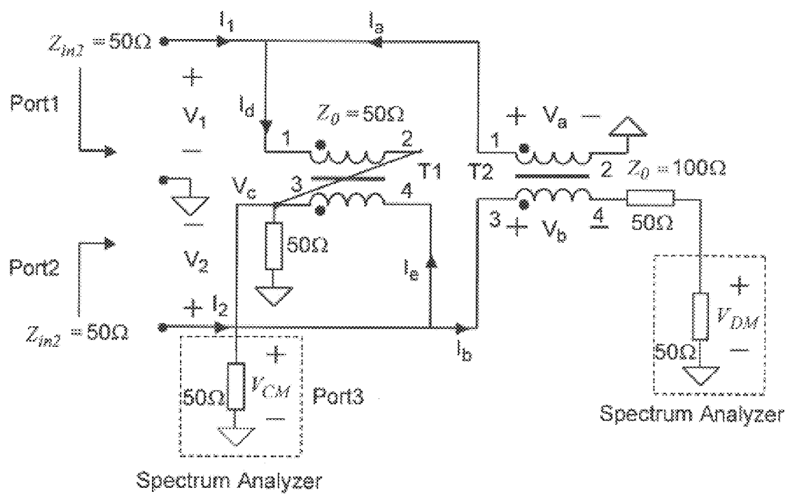
Figure 9 PRIOR ART
