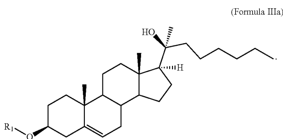
(Formula IIIa)
