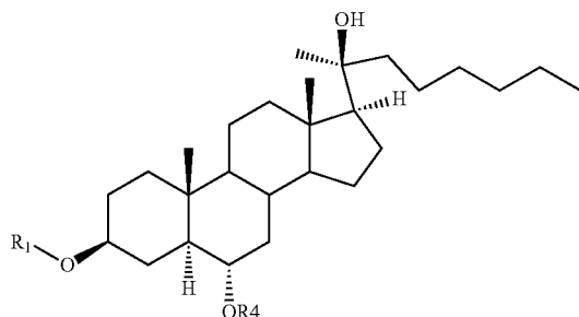
(Formula V)
