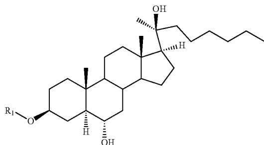
(Formula Va)
