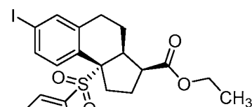
Intermediate 1
