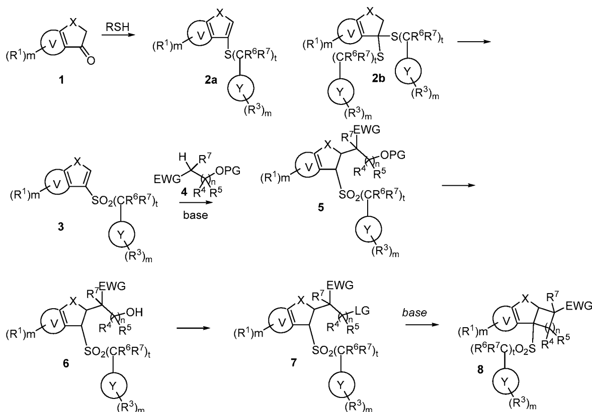
SCHEME 1
