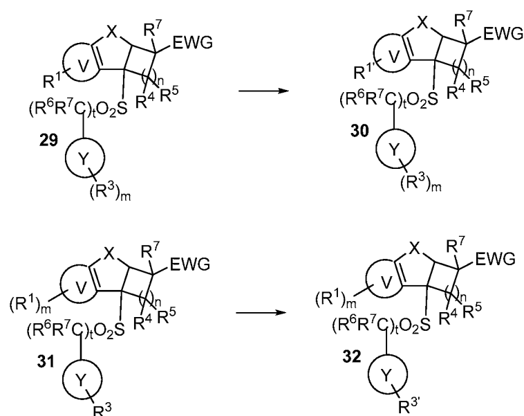
SCHEME 8
