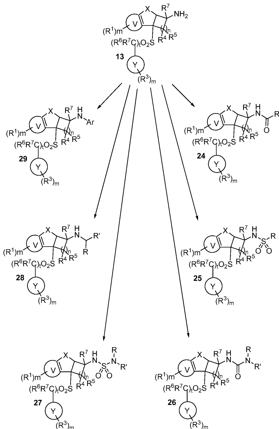
SCHEME 7
