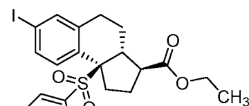
Intermediate 2
