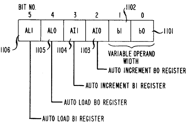
OP-CODE EXTENSION REGISTER BIT ASSIGNMENT:
