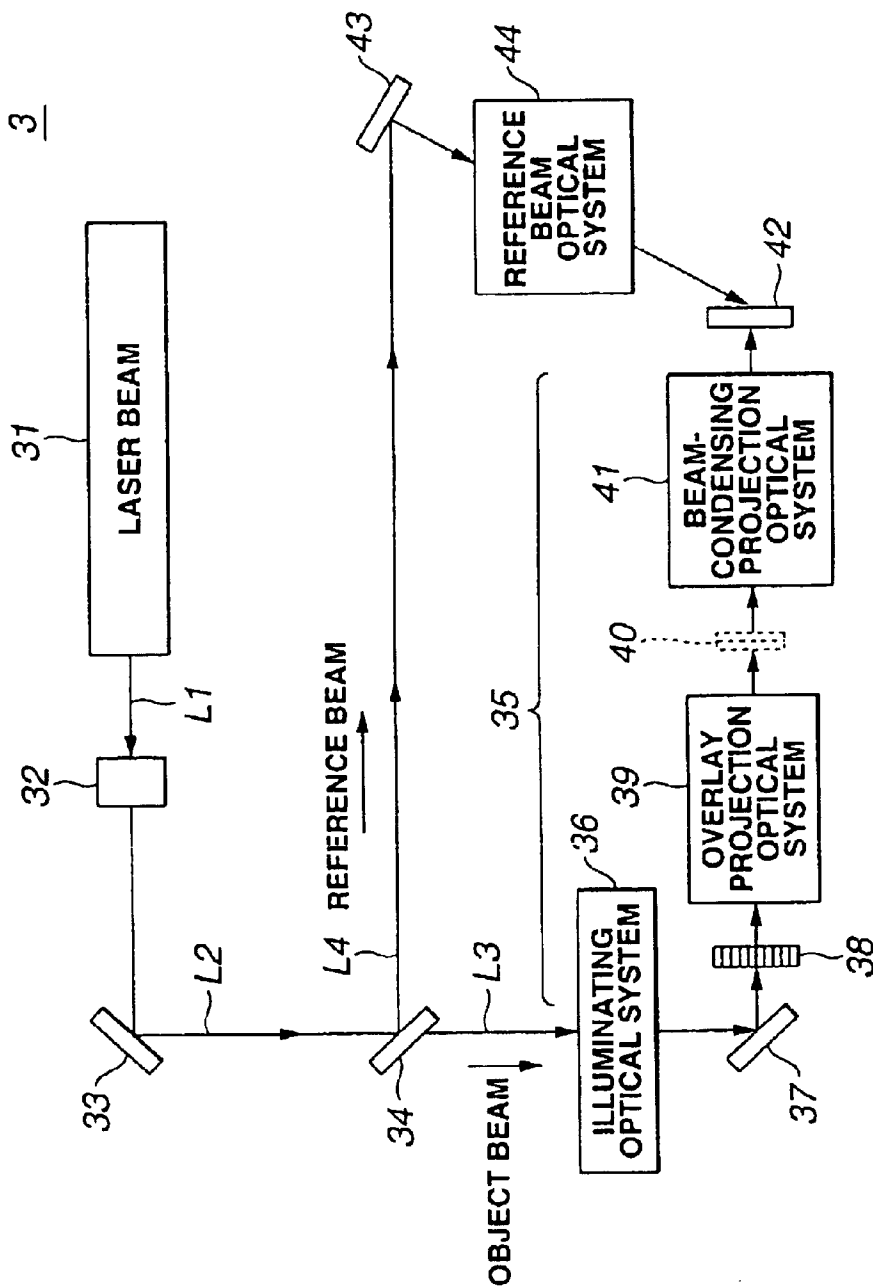
3 : HOLOGRAPHIC STEREOGRAM EXPOSURE APPARATUS 35 : OBJECT BEAM OPTICAL SYSTEM
