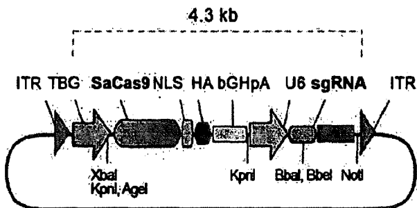
Liver-specific AAV-Sa-Cas9 vector: TBG-SaCas9-NLS-HA-U6-sgRNA
