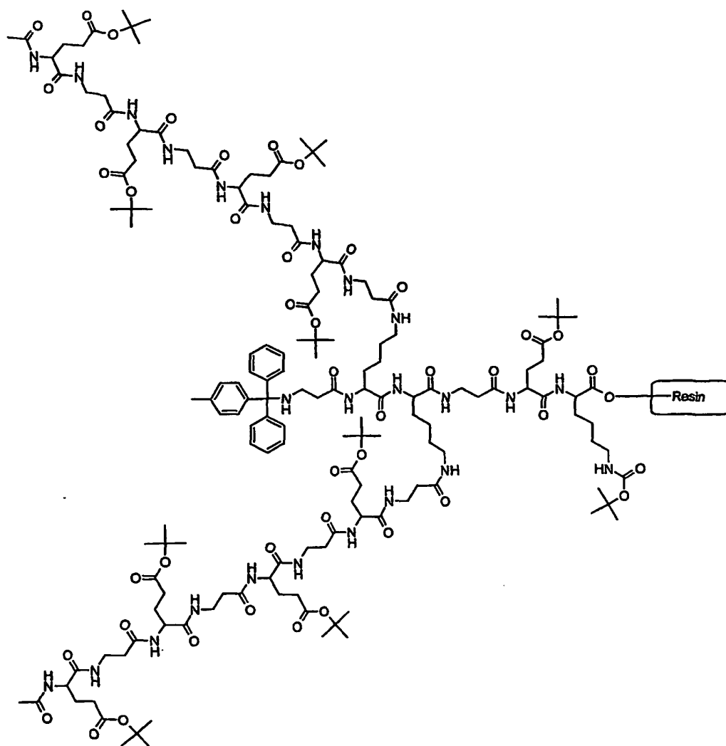
Figure 21: Solid-phase bound branched linker (with protective groups)
