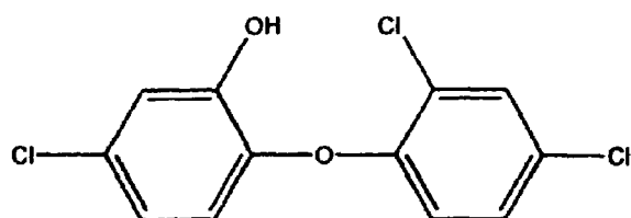
2,4,4'-trichloro-2'-hydroxy diphenol ether
