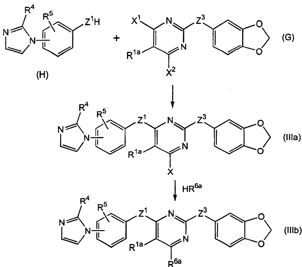
Reaction Scheme 4
