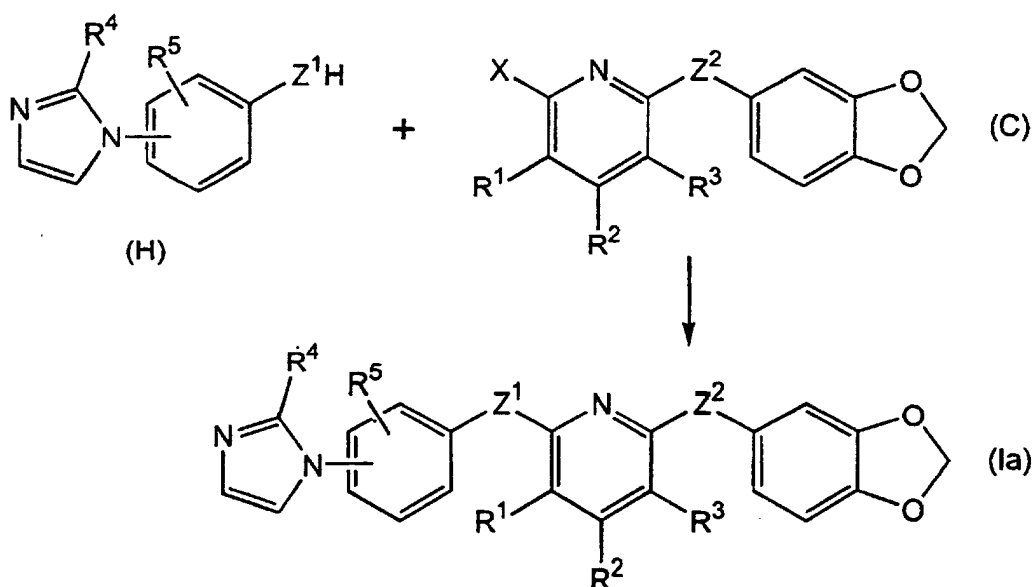
Reaction Scheme 3
