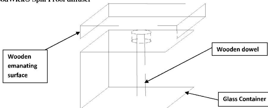
WoodWick® Spill Proof diffuser
