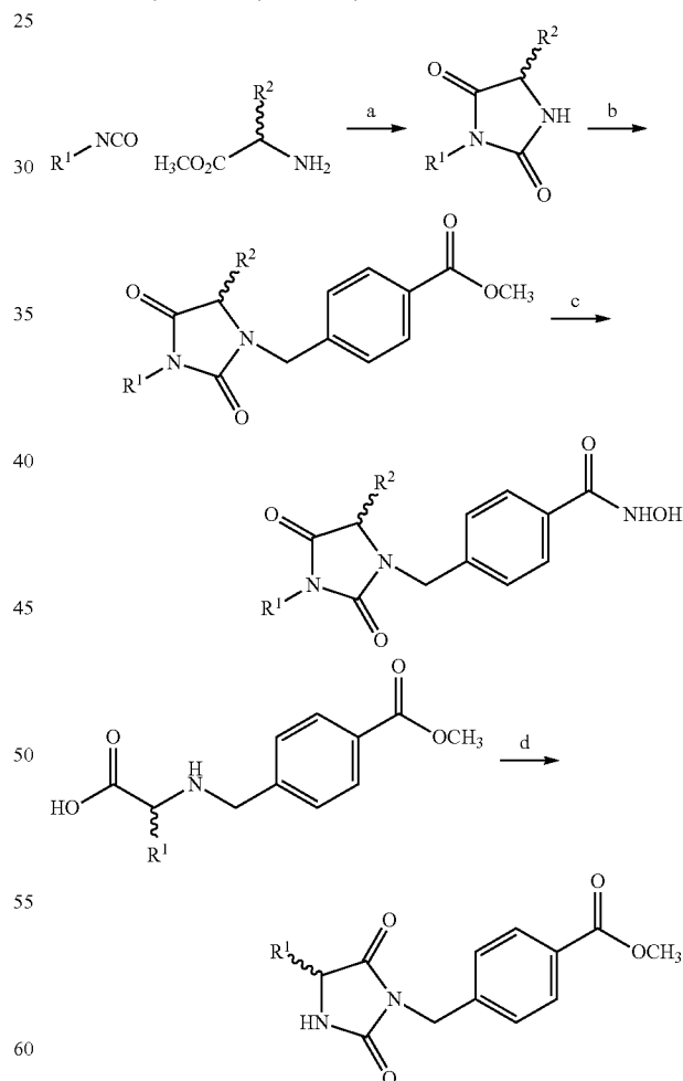
Scheme 3: Synthesis of cyclic urea hydroxamic acids
