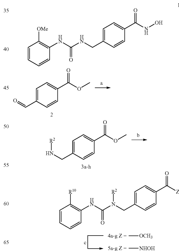
Scheme 1: Synthesis of proximal N-substituted hydroxamic acids
