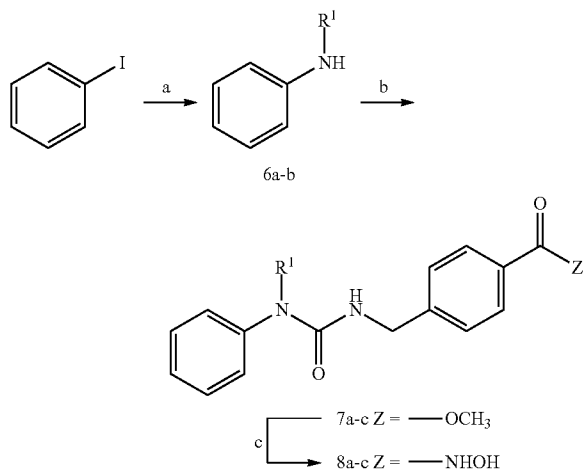
Scheme 2: Synthesis of distal N-substituted hydroxamic acids
