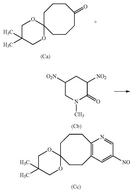
REACTION SCHEME 2
