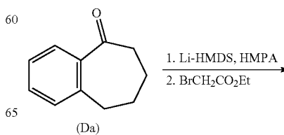
REACTION SCHEME 3
