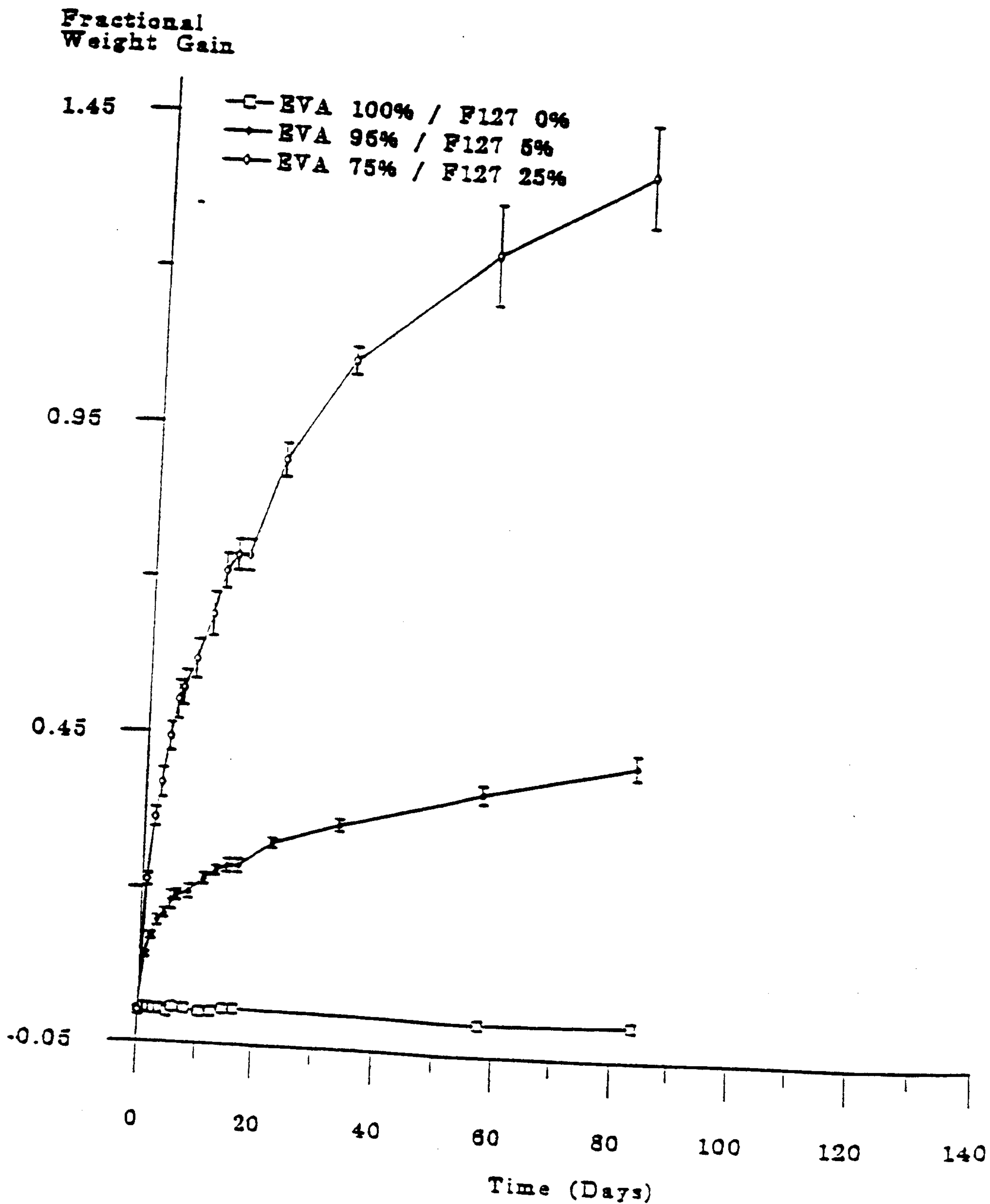
Swelling of EVA/F127 Films with no Taxol
