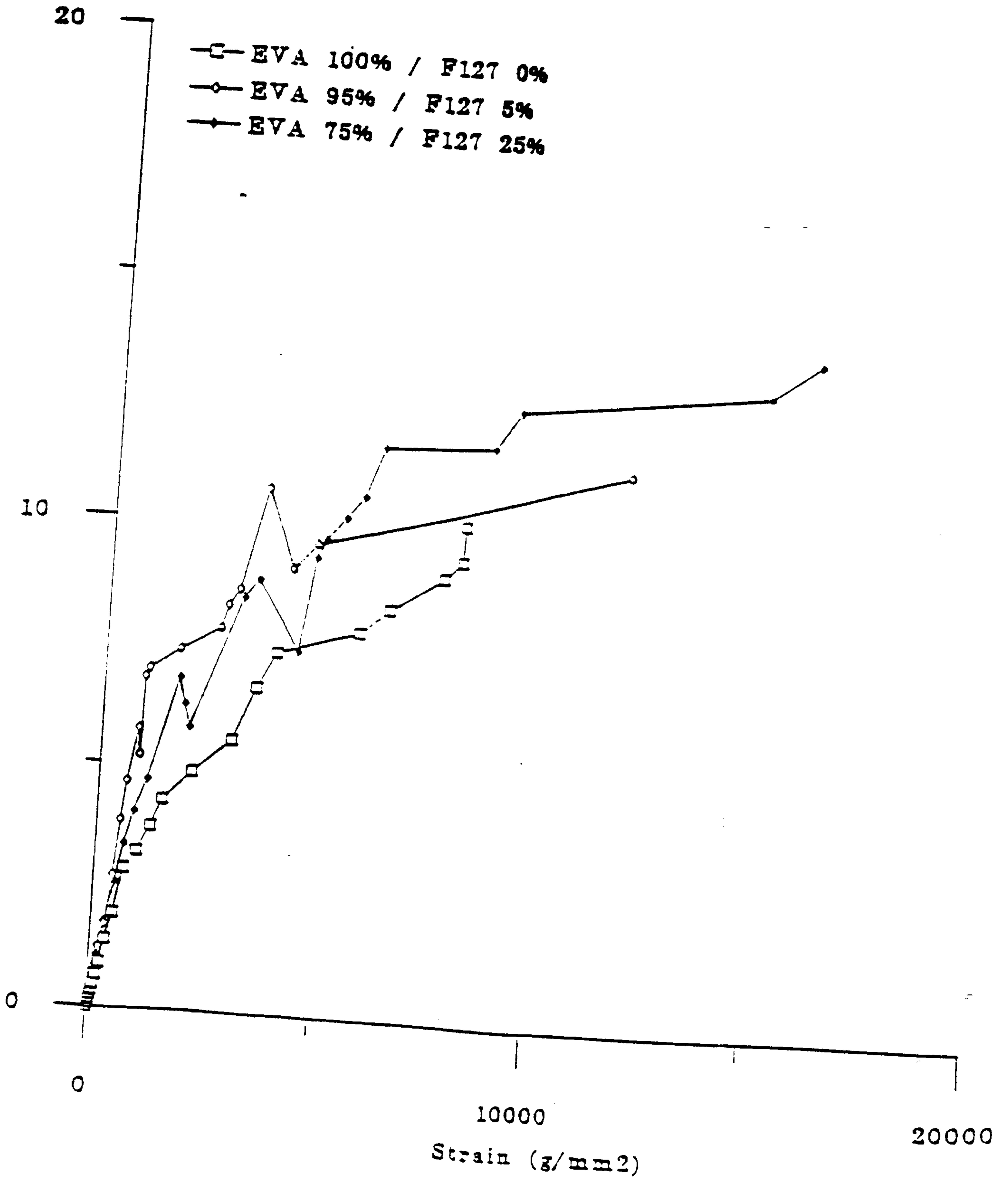
Stress/Strain Curve of EVA and Blend Films Containing EVA/F127
