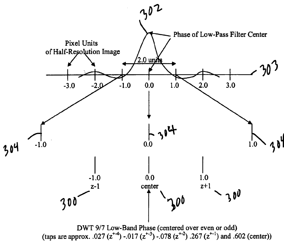
Fig. 3 (Prior Art)
