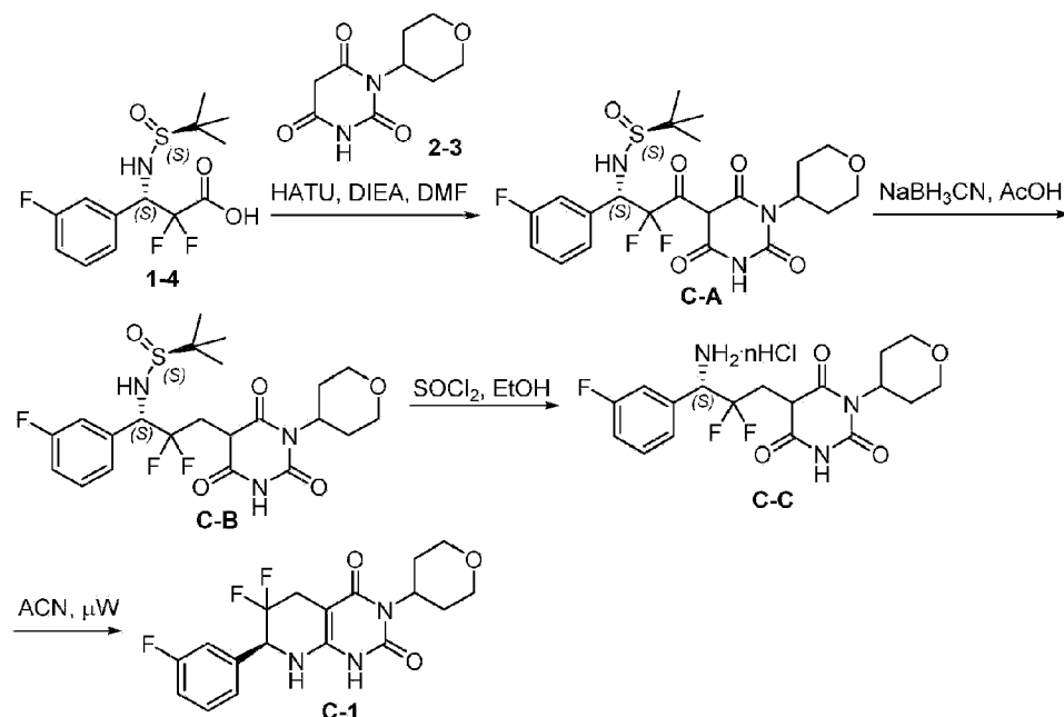
Scheme C-1
