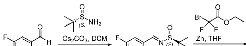
Scheme I-1
