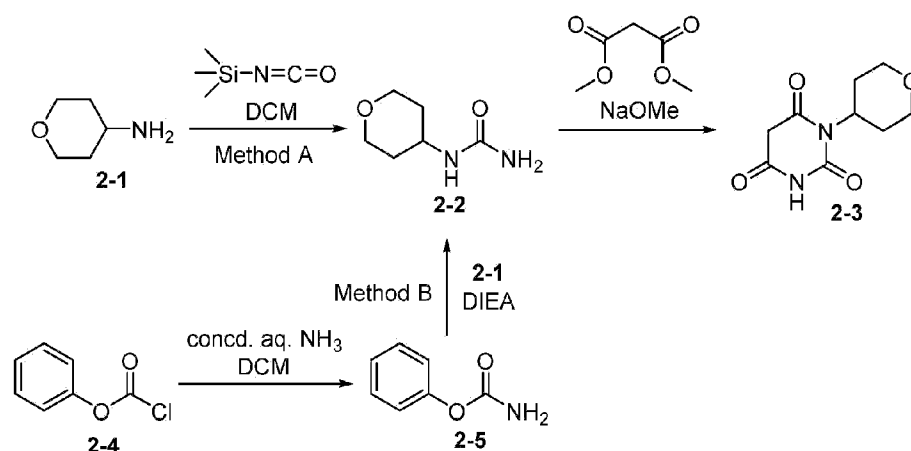
Scheme I-2
