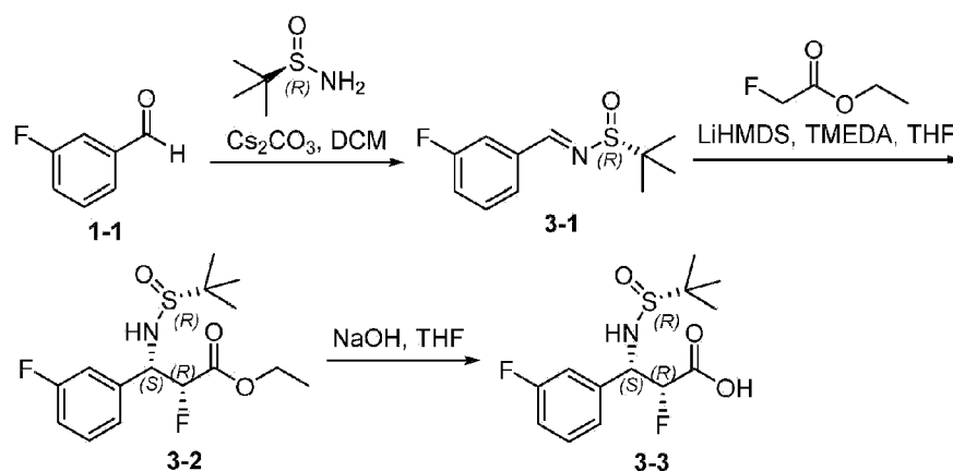
Scheme I-3
