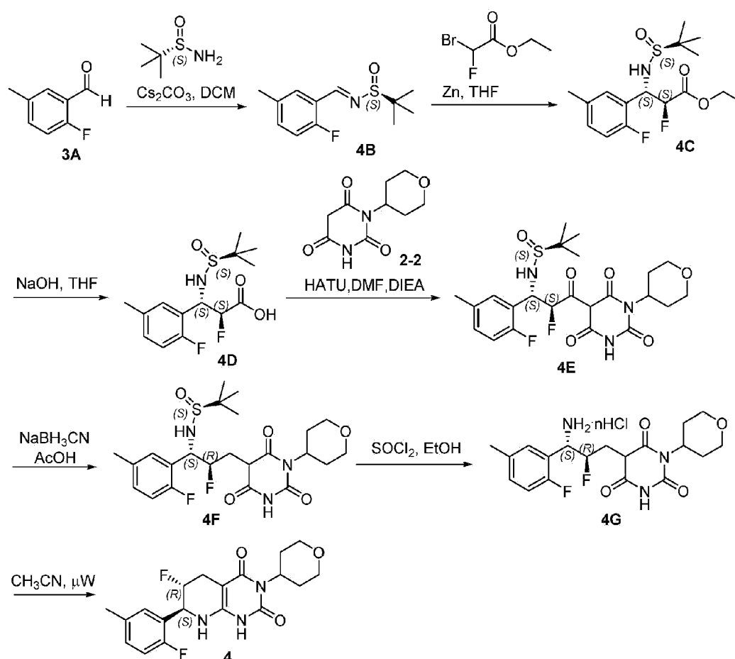
Scheme 4
