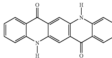
quinacridone (green light emission)
