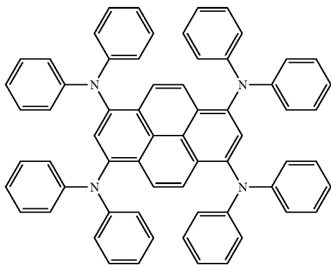
1,3,6,8-tetrakis(diphenylamino)pyrene (green light emission)
