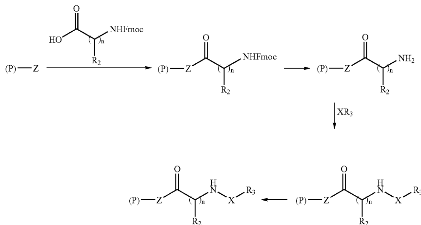
Reaction Scheme 2
