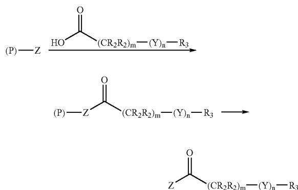
Reaction Scheme 1.
