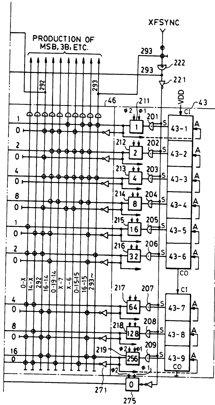
CIRCUIT B OF FIG. 5
