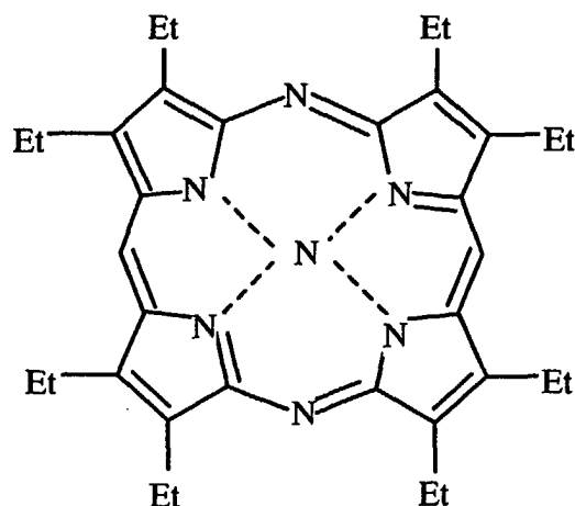
Chemical formula 2
