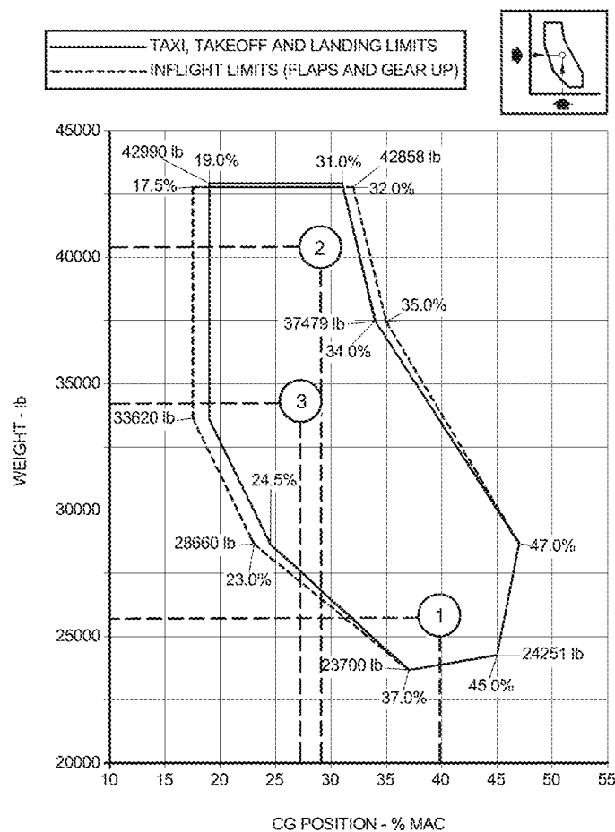
COMPUTATION OF CG - EXAMPLE
