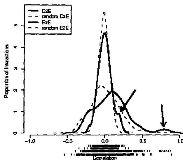
Fig. 1. NCI Pathway interactions in TCGA GBM data. For all ( n=462 ) pairs where A was found to be an upstream activator of gene B in NCI-Nature Pathway Database, the Pearson correlation ( x -axis) computed from the TCGA GBM data was calculated in two different ways. The histogram plots the correlations between the A's copy number and B's expression (C2E, solid red) and between A's expression and B's expression (E2E, blue). A histogram of correlations between randomly paired genes is shown for C2E (dashed red) and E2E (dashed blue). Arrows point to the enrichment of positive correlations found for the C2E (red) and E2E (blue) correlation.
