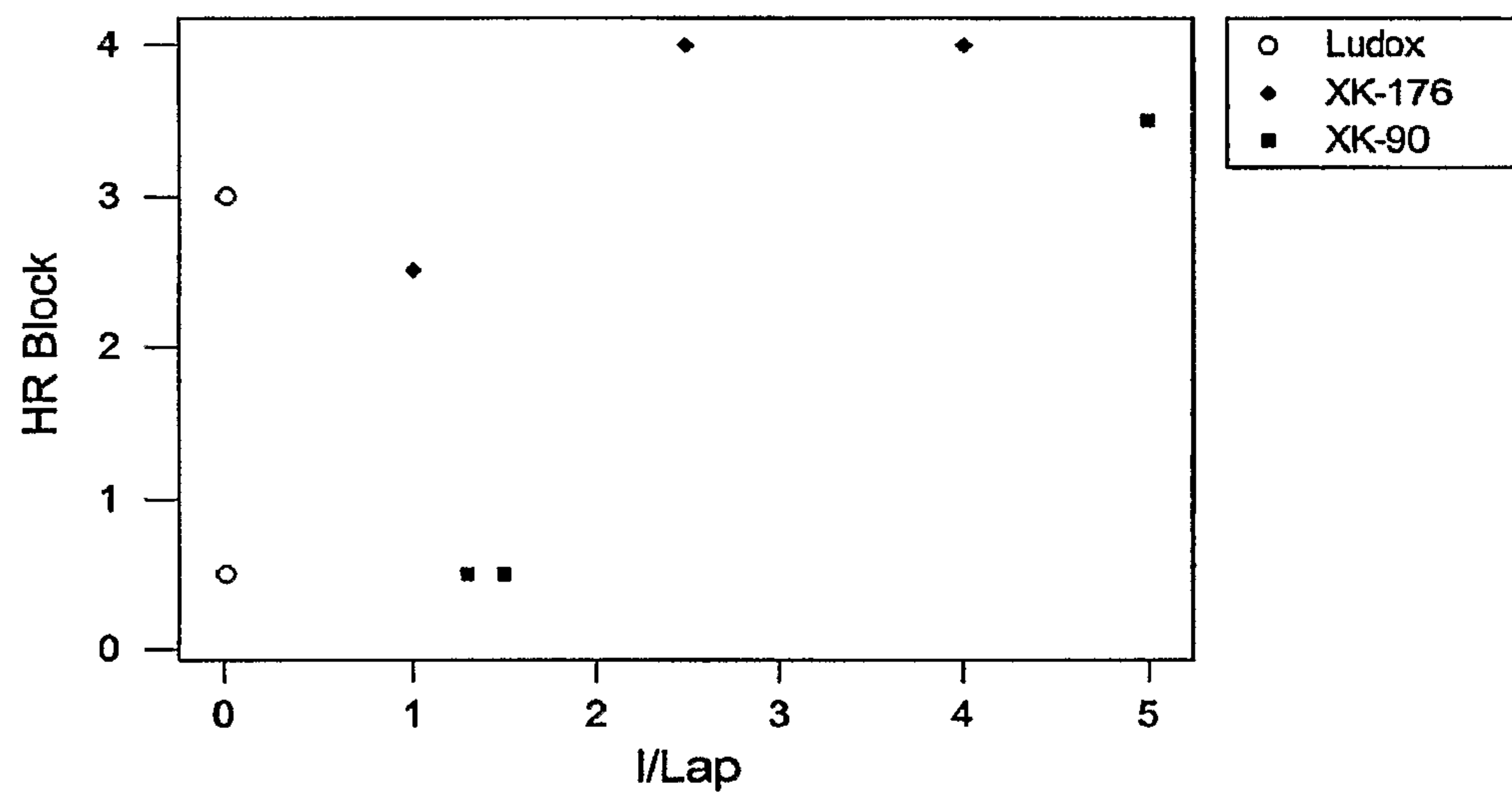
Blocking Rating versus NeoCryl/Laponite Ratio
