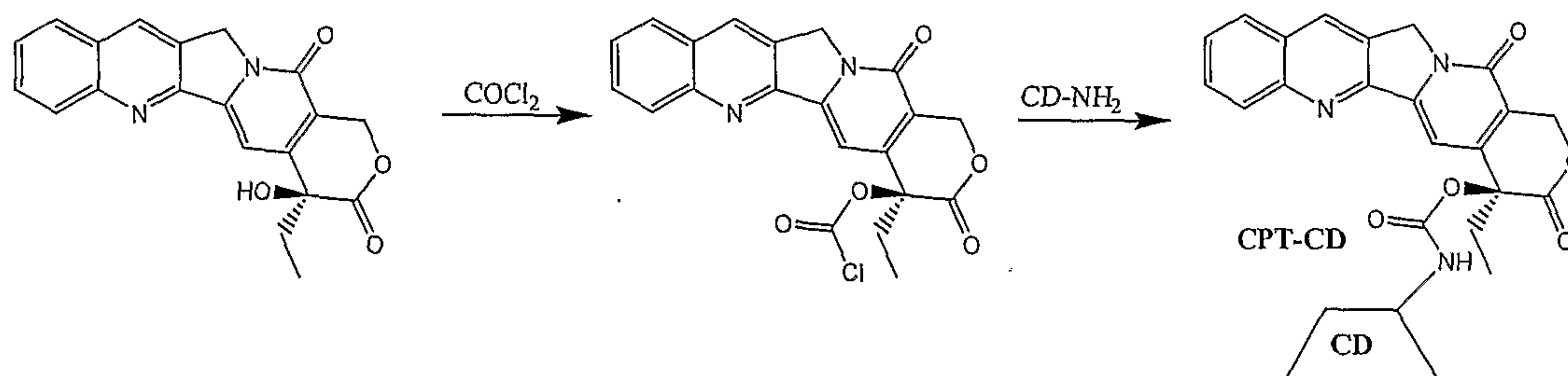
Scheme I
