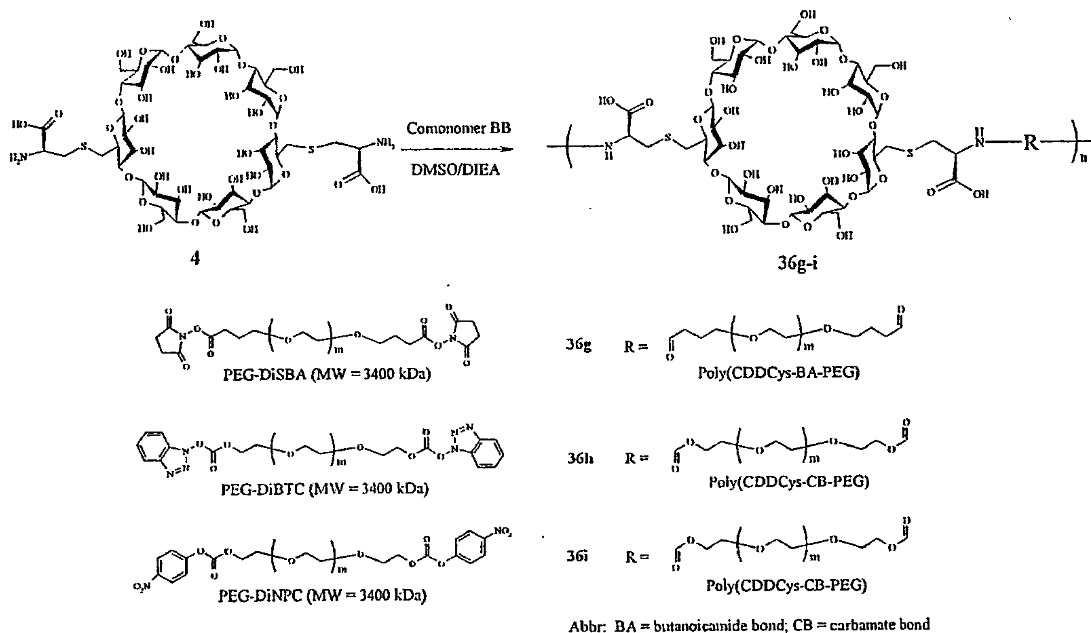
Scheme XXXVIIIb
