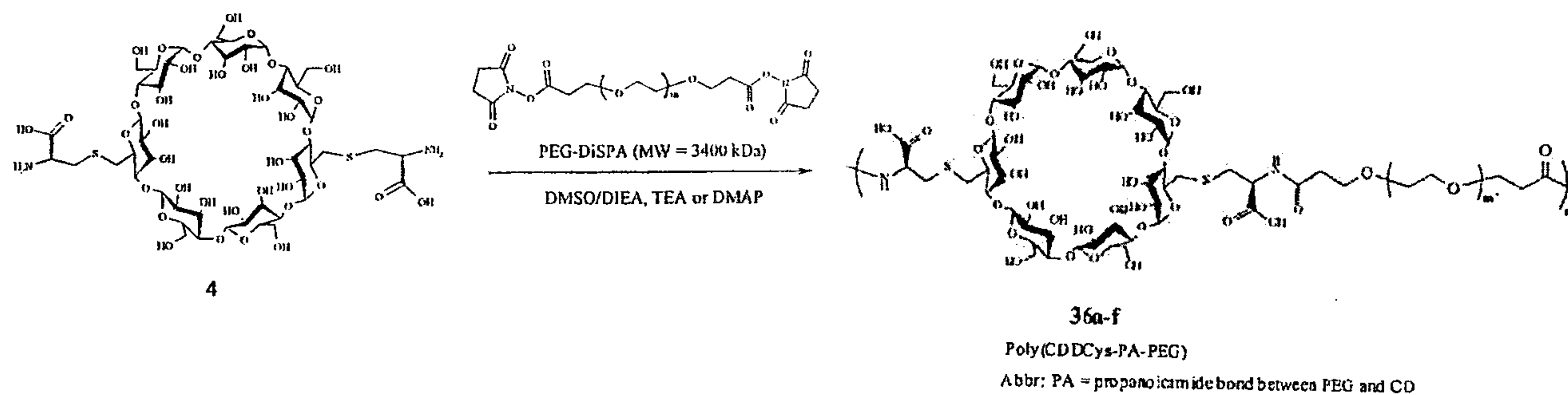
Scheme XXXVIIIa
