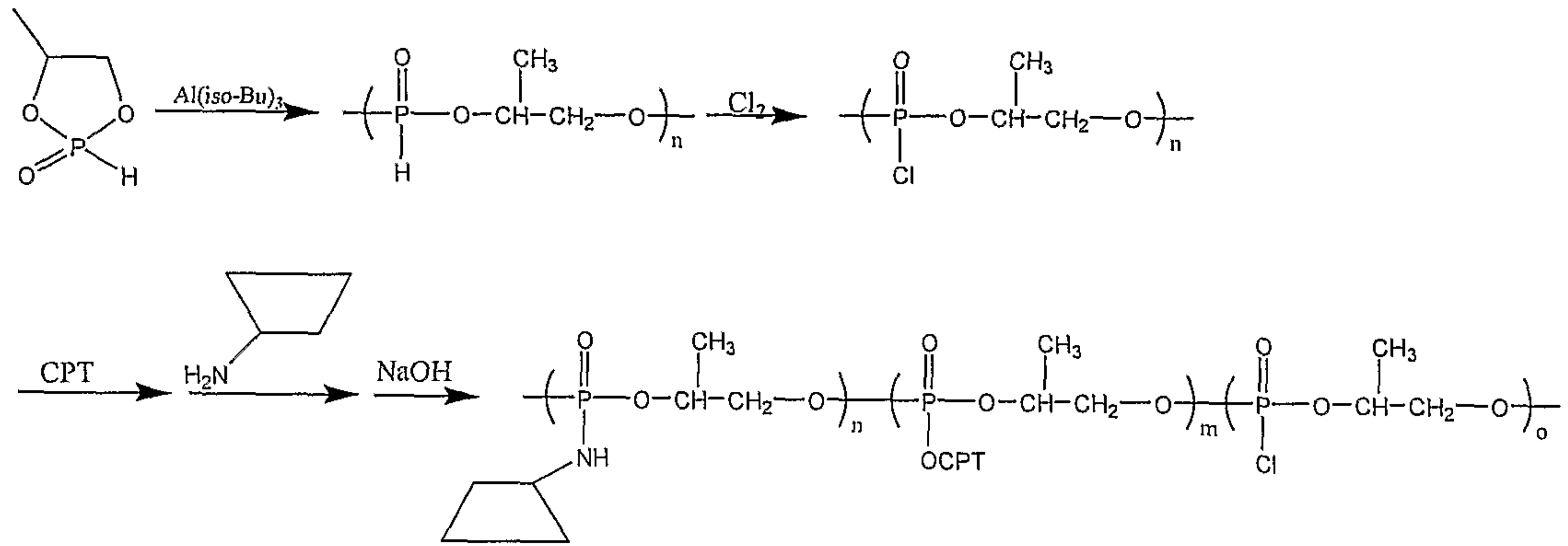
Scheme IX
