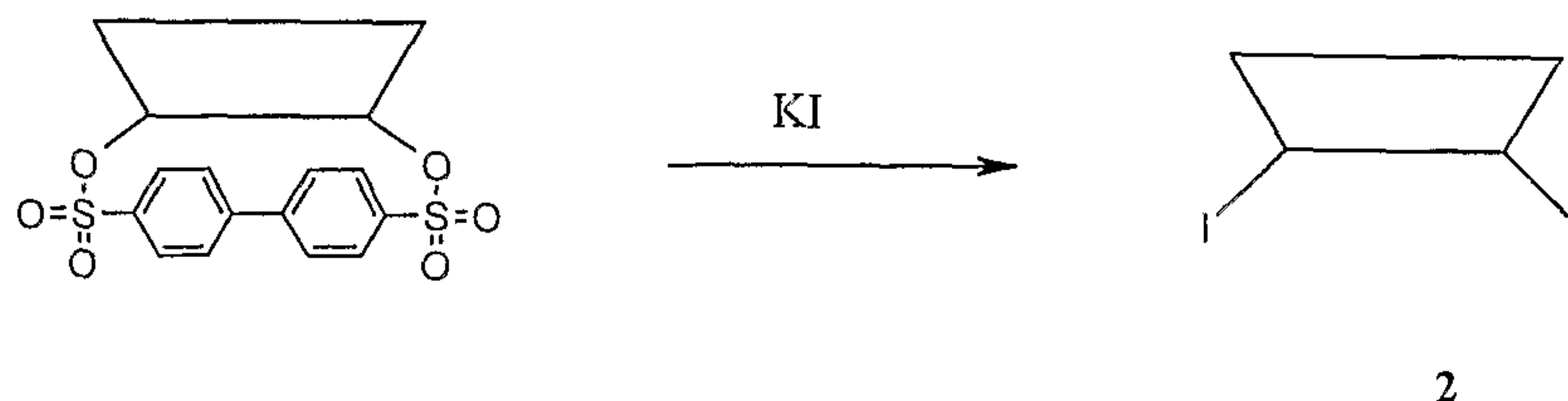
Scheme XVI
