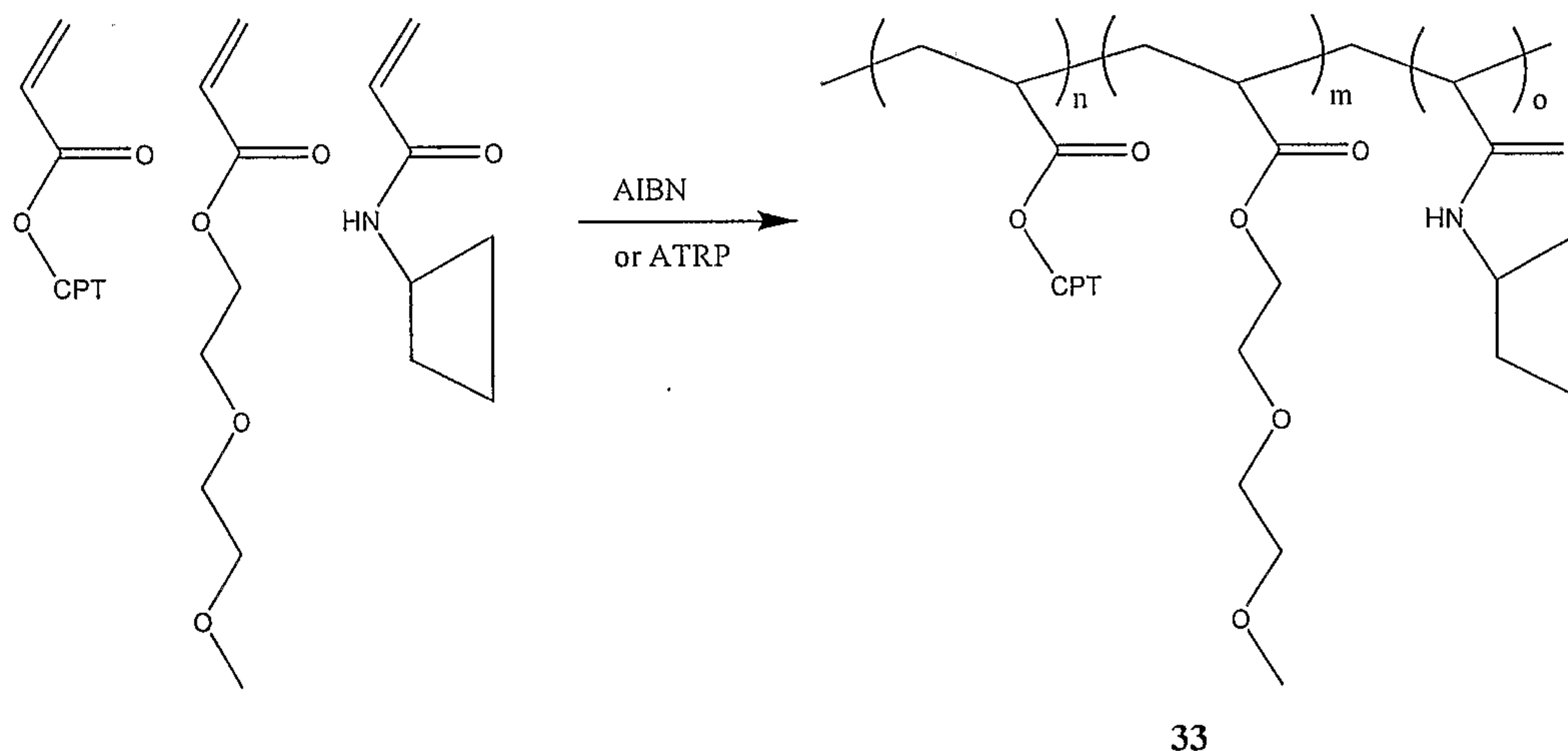
Scheme XXXV
