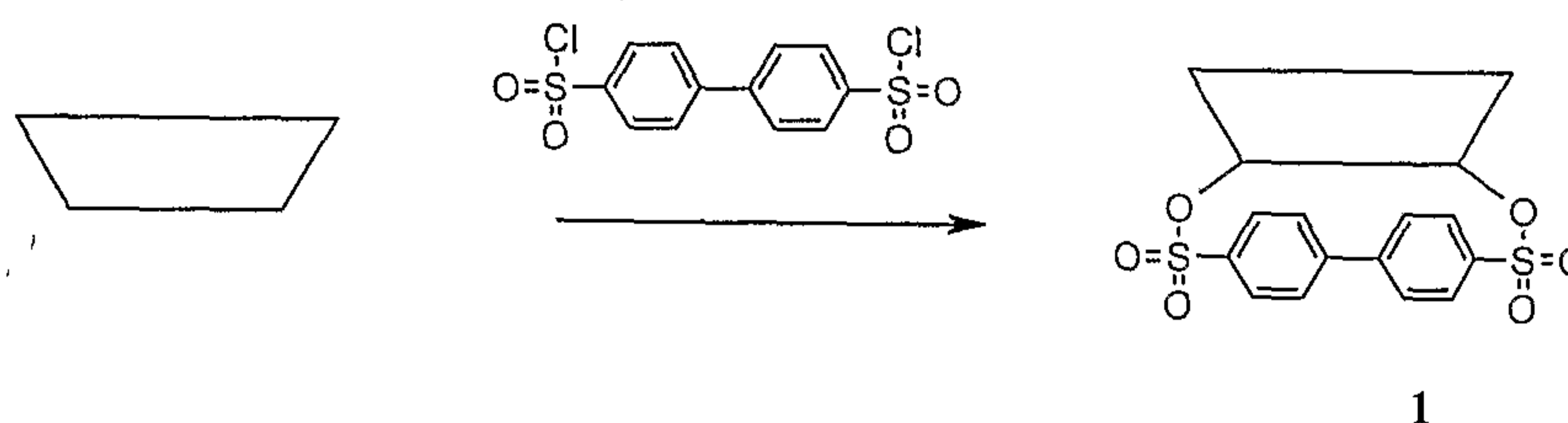
Scheme XV
