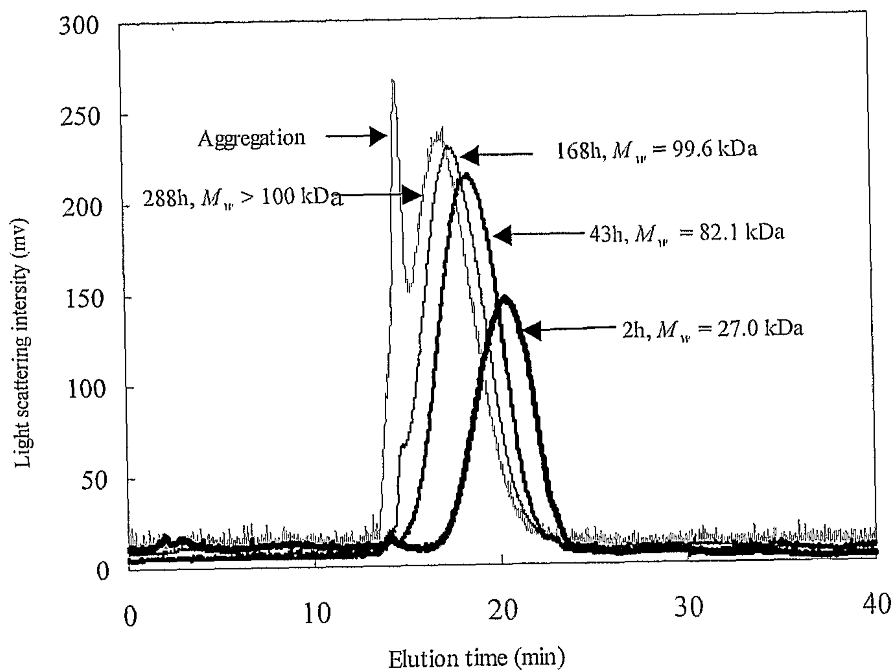
FIG. 5b: Polymerization control by adjusting polymerization time.
