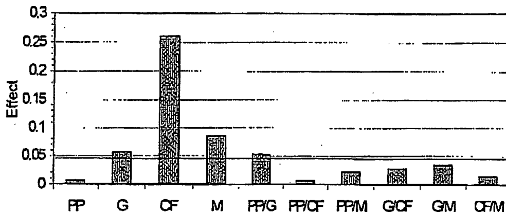
Pareto Chart for Coefficient of Friction
