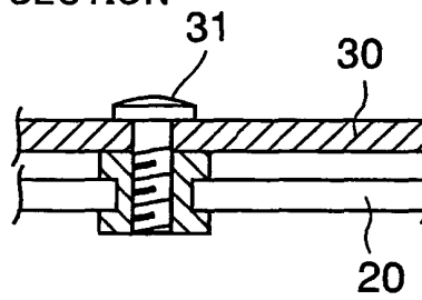
(B) B-B CROSS-SECTION
