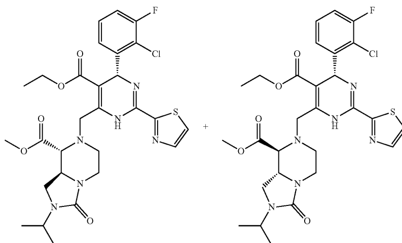
84A-1 &amp; 84B-1 (2 single isomers)
