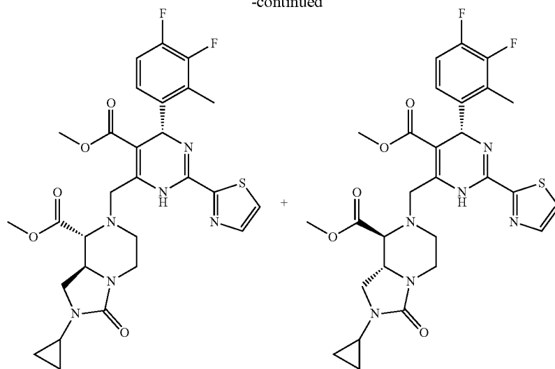
83A-1 &amp; 83B-1 (2 single isomers)
