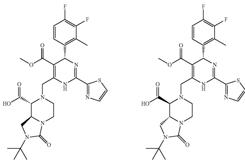
88A &amp; 88B
