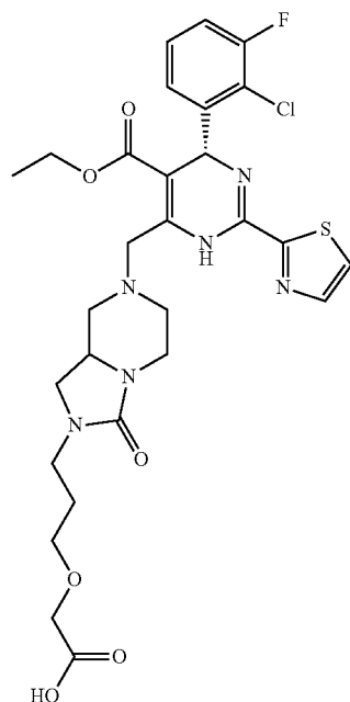
Preparation of Example 68
