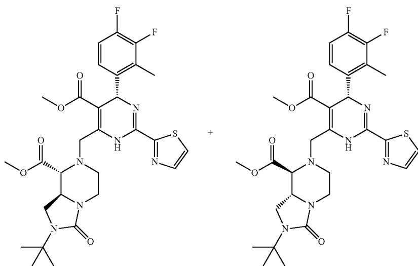
88A-1 &amp; 88B-1 (2 single isomers)
