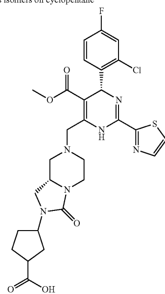
63 mixture of two trans isomers on cyclopentane
