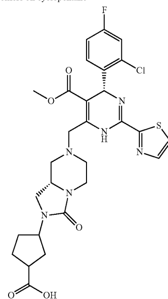
61 mixture of two cis isomers on cyclopentane
