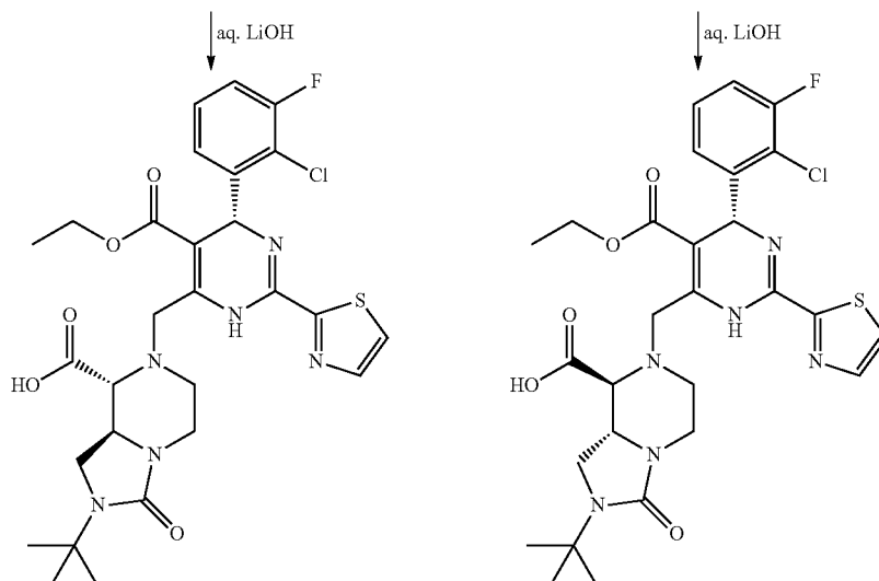
87A &amp; 87B
