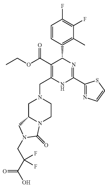
Preparation of Example 96
