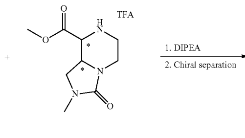
91-C mixture of two trans isomers
