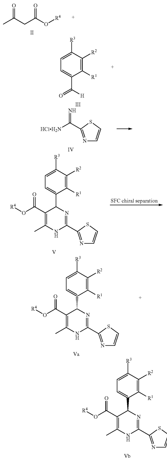
Scheme 1
