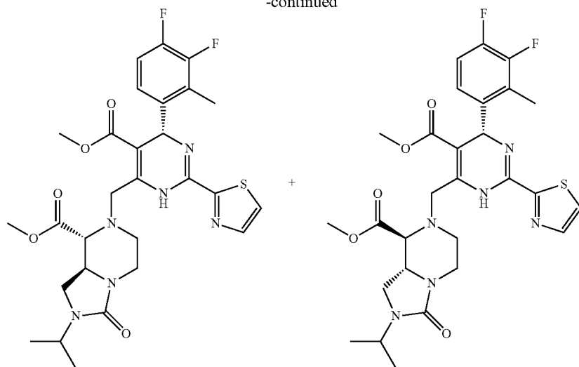
85A-1 &amp; 85B-1 (2 single isomers)
