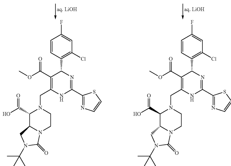
86A &amp; 86B
