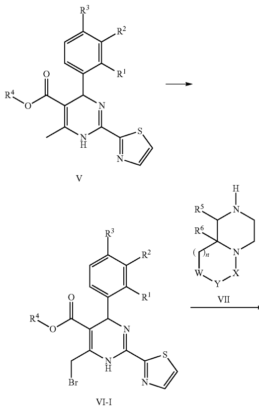
Scheme 1-1
