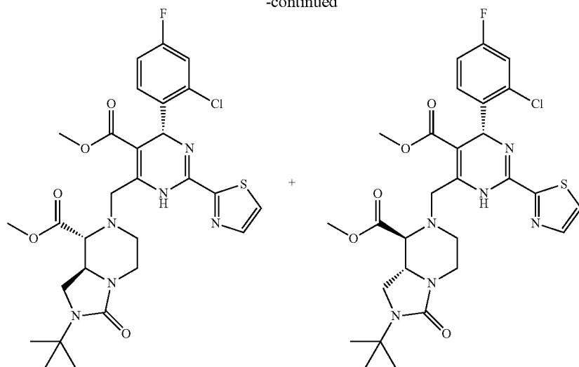
86A-1 &amp; 86B-1 (2 single isomers)
