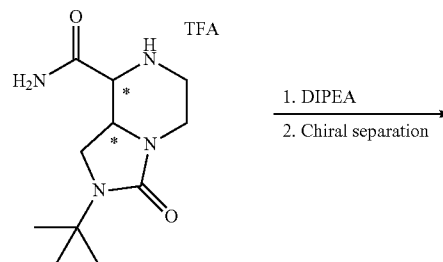
92-C mixture of two trans isomers
