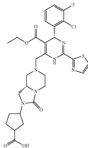
62 mixture of two cis isomers on cyclopentane
