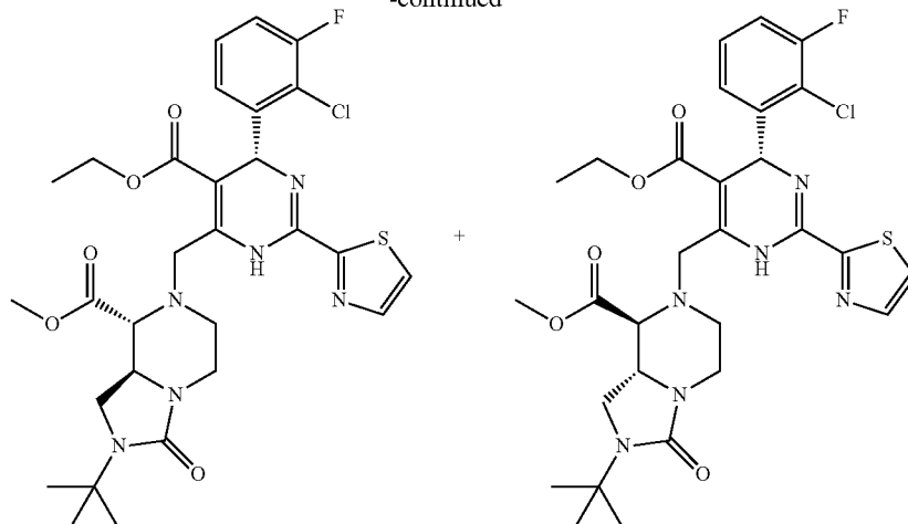
87A-1 &amp; 87B-1 (2 single isomers)
