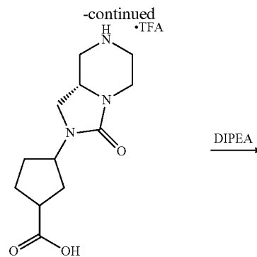
61-A mixture of two cis isomers on cyclopentane
