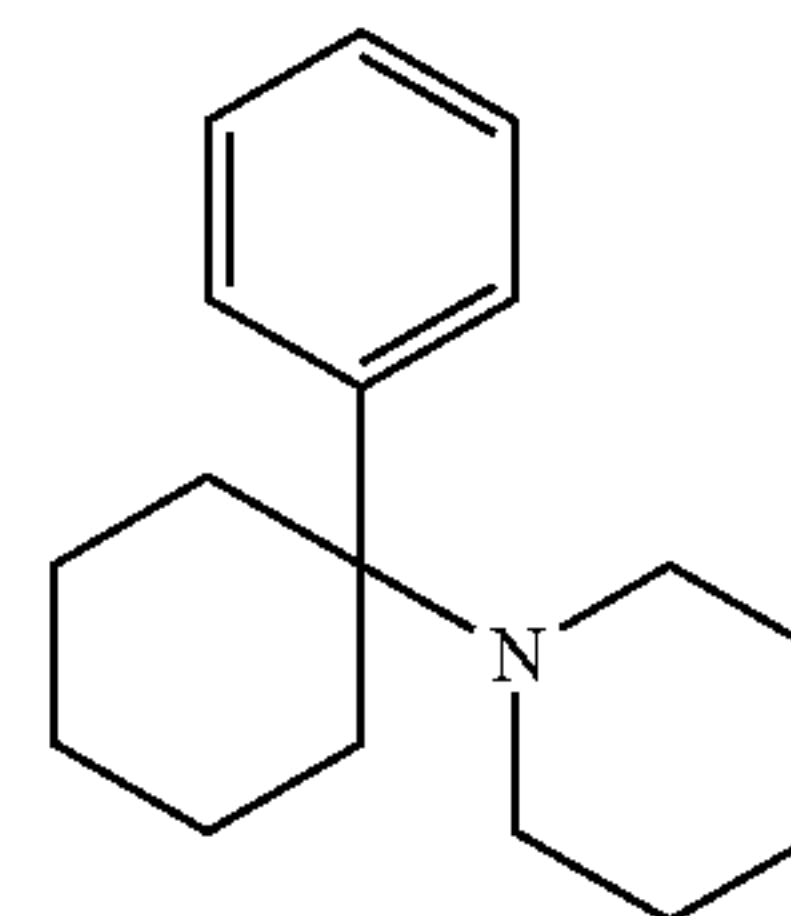
Phencyclidine (PCP)
