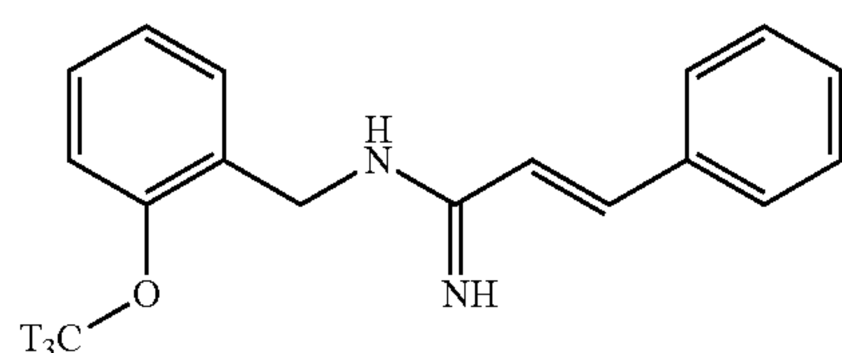
[ ^3\text{H} ] (E)-N1-(2-methoxybenzyl)-cinnamidine
