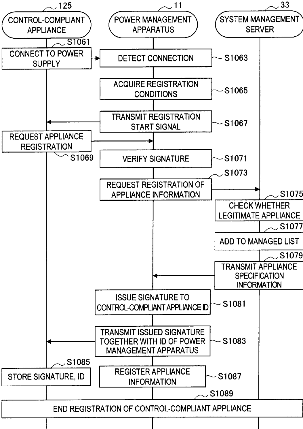
(INITIAL REGISTRATION OF CONTROL-COMPLIANT APPLIANCE)
