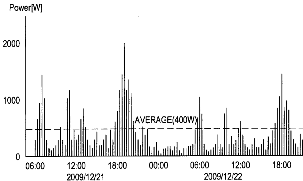
(A) EXAMPLE OF POWER CONSUMPTION PATTERN
