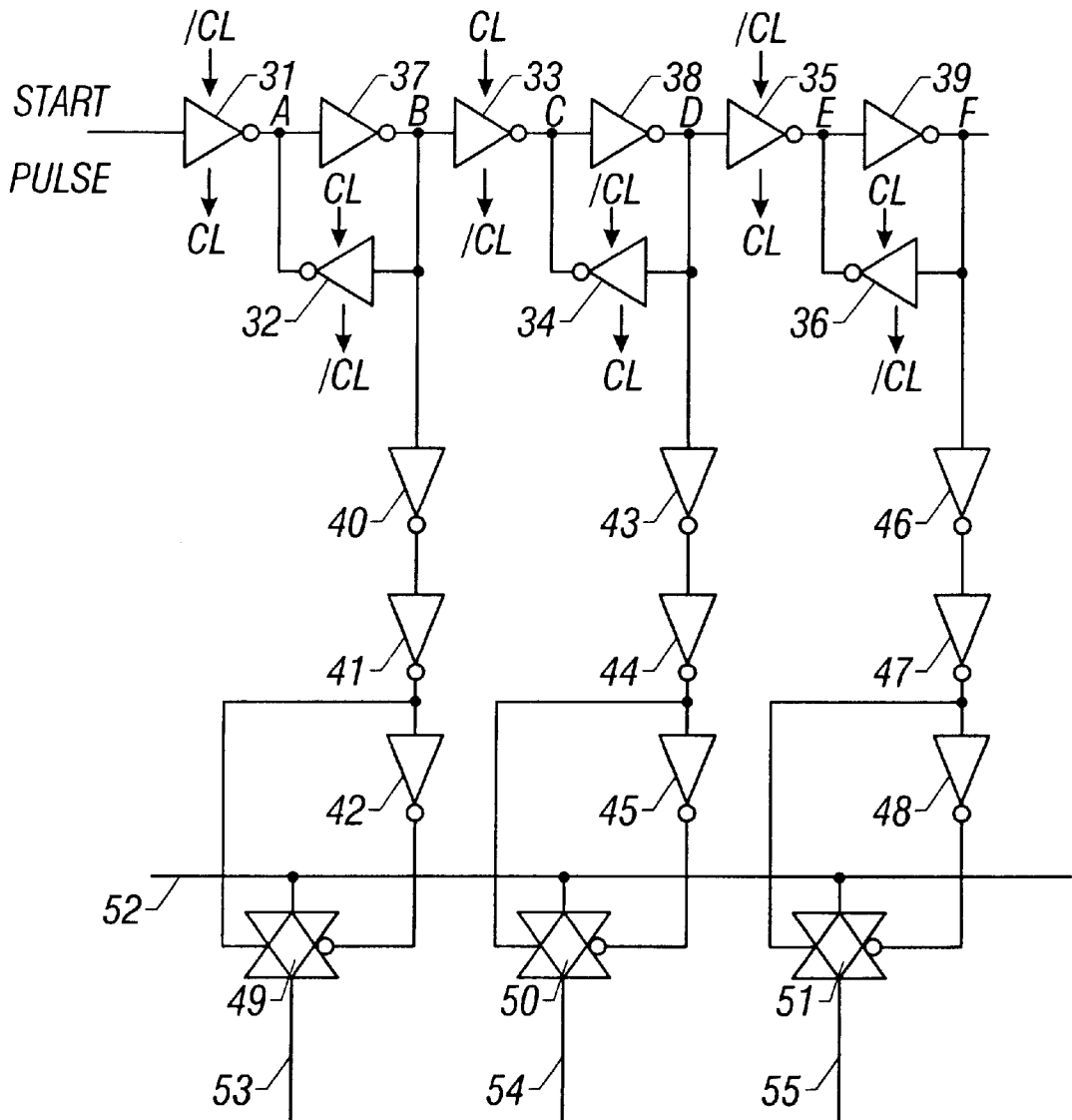
FIG. 25A (Prior Art)
