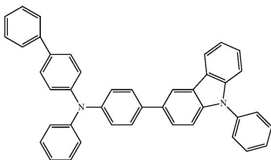
PCBA1BP
