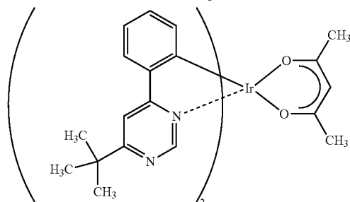
[Ir(tBuppm) 2 (acac)]
