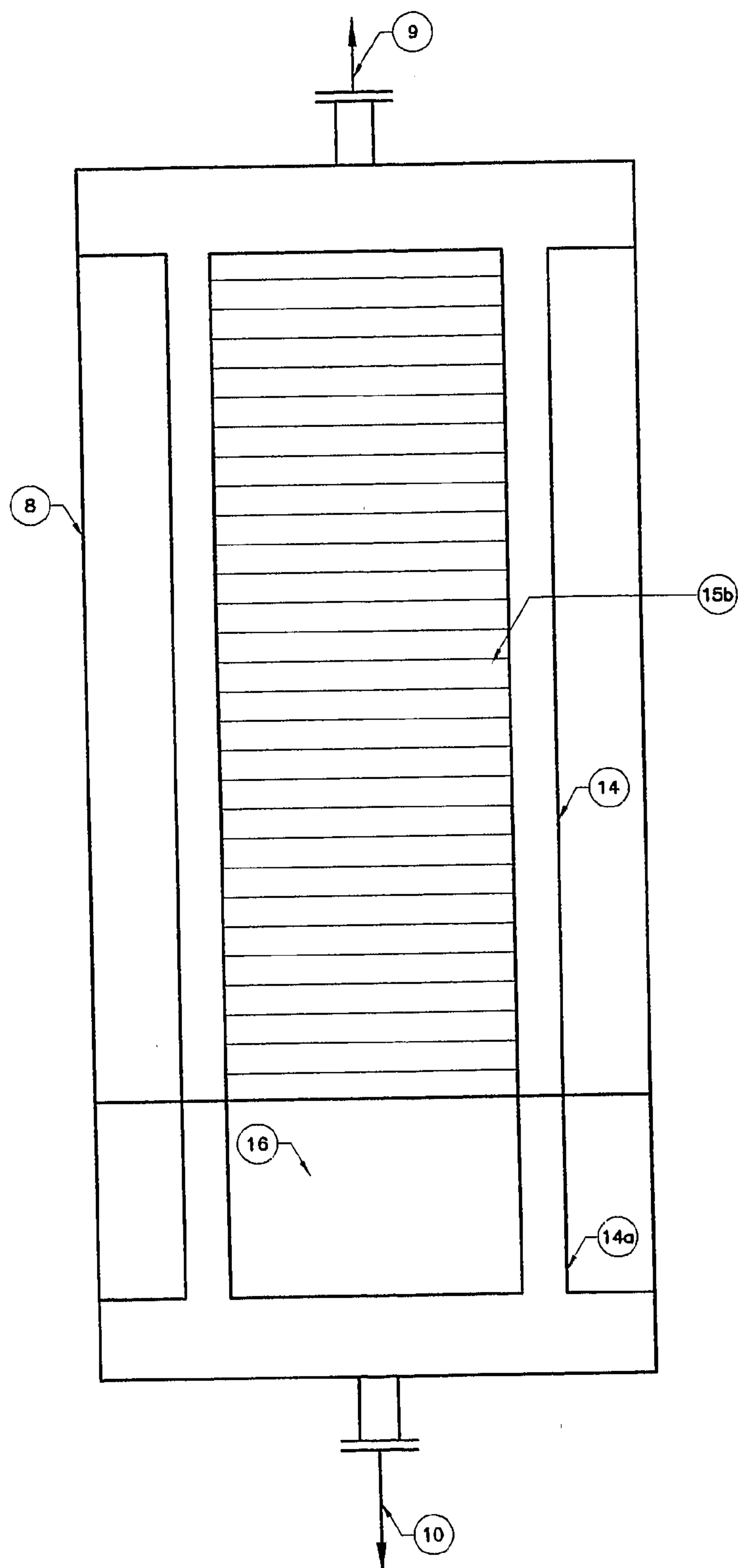
FIGURE 2c. THREE PHASE SEPARATOR (TOP VIEW)
