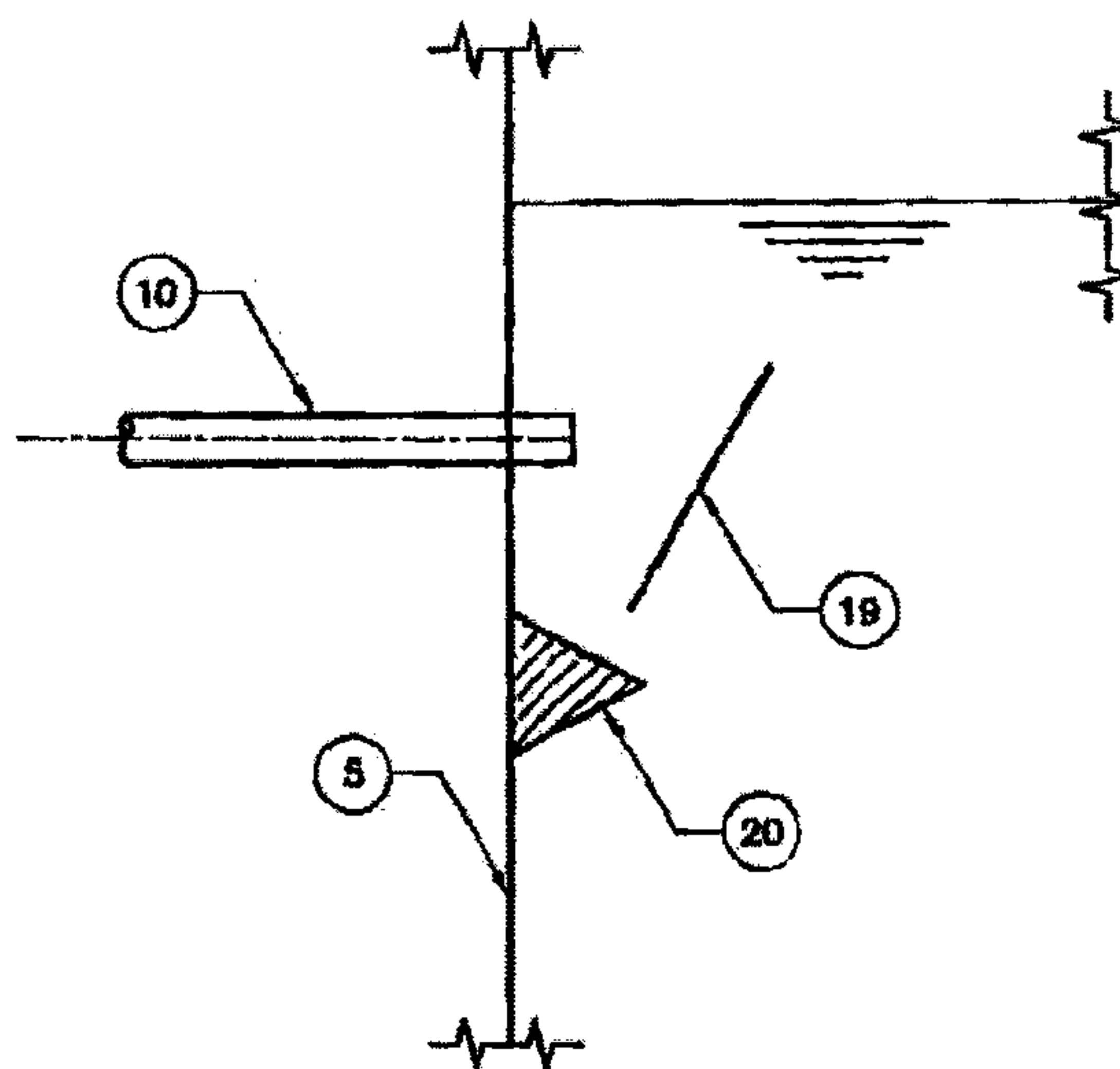
FIGURE 6. GAS DEFLECTING DEVICE
