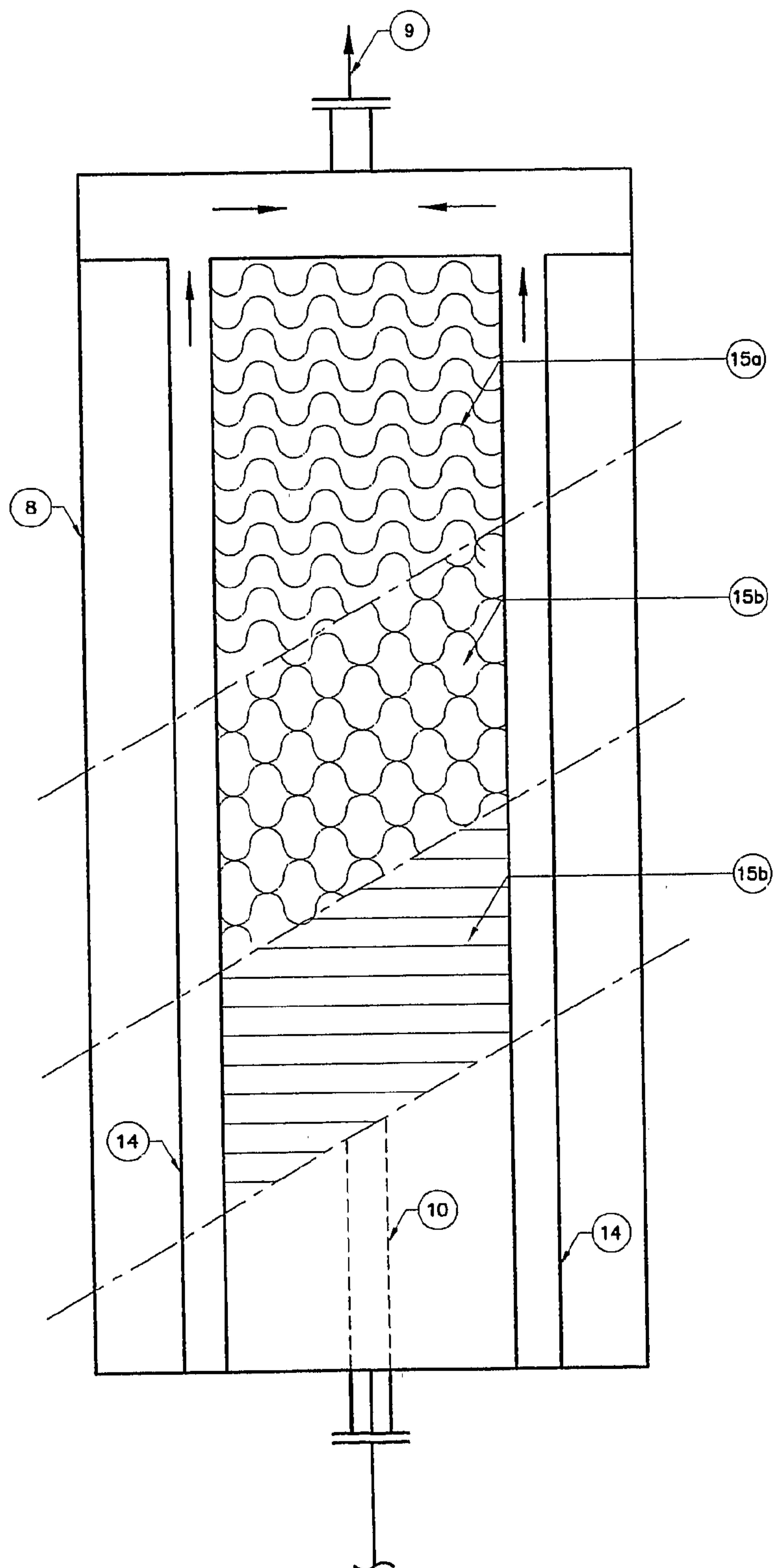
FIGURE 2b. THREE PHASE SEPARATOR (TOP VIEW)
