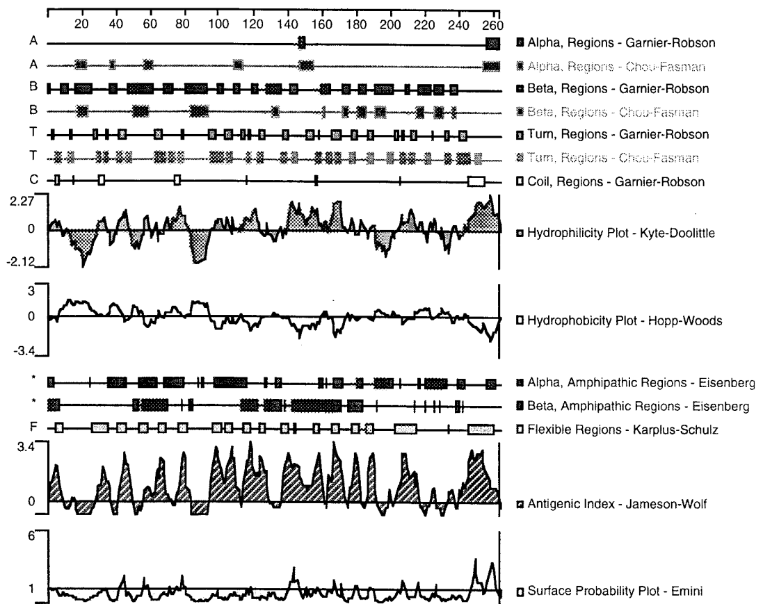
Figure 3 Follistatin-3
