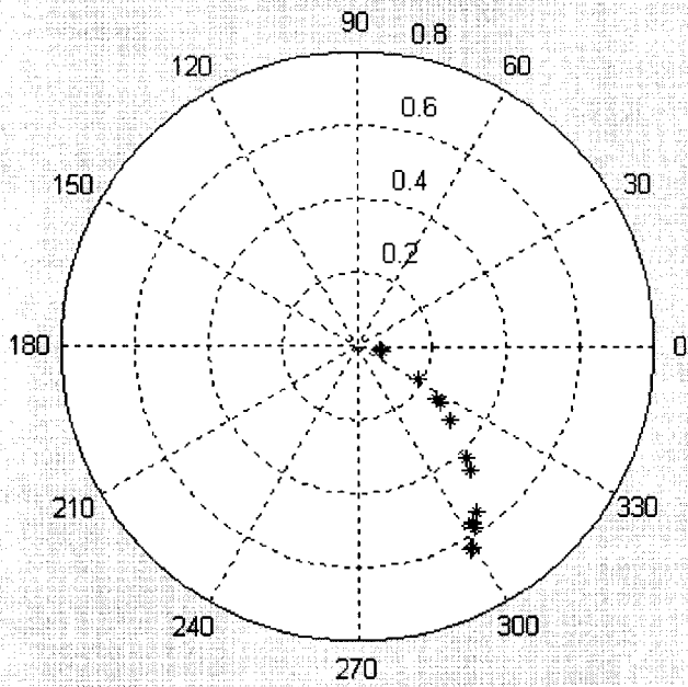
Reflection coefficient for the 3.1 mm deflector, deflector angle as parameter, 2455 MHz
