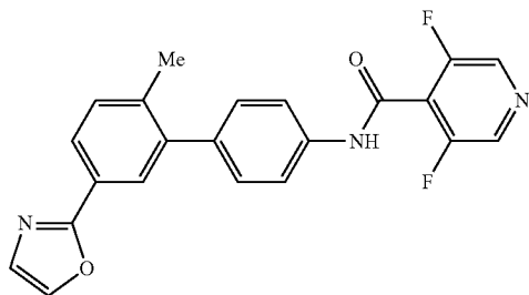
Compound 11: 3,5-Difluoro-N-(2'-methyl-5'-oxazol-2-yl-biphenyl-4-yl)-isonicotin-amide
