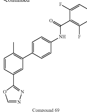
Compound 46: 3-Methyl-N-[2'-methyl-5'-([1,3,4]oxadiazol-2-yl)-biphenyl-4-yl]-isonicotinamide, HCl salt
