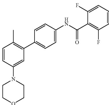
Compound 43
