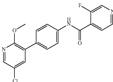
Compound 19: 3-Fluoro-N-[4-(5-chloro-2-methoxy-pyridin-3-yl)-phenyl]-isonicotinamide
