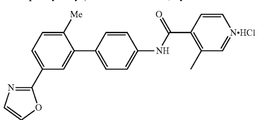
Compound 7: 3-Methyl-N-(2'-methyl-5'-oxazol-2-yl-biphenyl-4-yl)-isonicotinamide, hydrochloride
