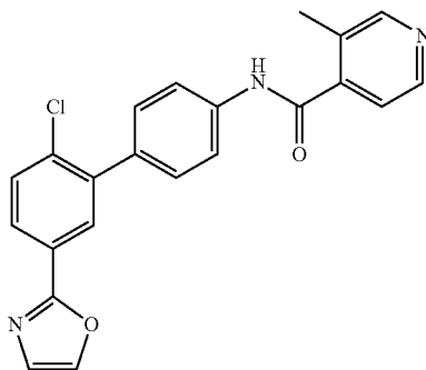
Compound 16: 3-Methyl-N-(2'-chloro-5'-oxazol-2-yl-biphenyl-4-yl)-isonicotinamide
