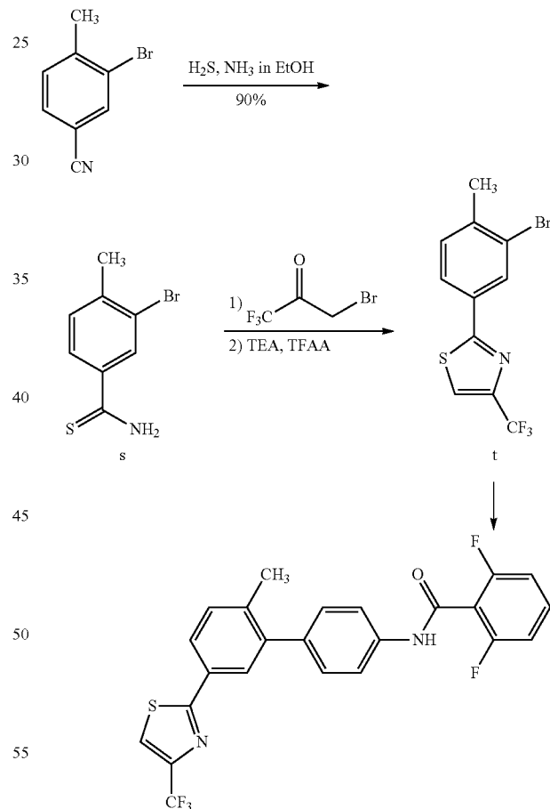
Compound 39
