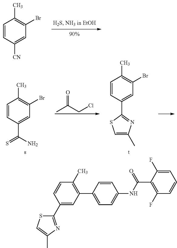
Compound 38
