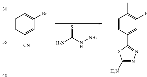
Scheme XXII
