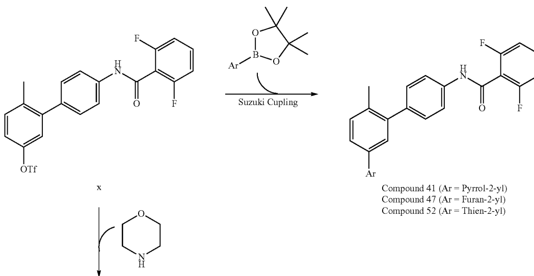
Scheme XVIII
