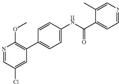
Compound 18: 3-Methyl-N-[4-(5-chloro-2-methoxy-pyridin-3-yl)-phenyl]-isonicotinamide
