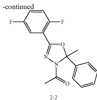
3-acetyl-5-(2,5-difluorophenyl)-2-methyl-2-phenyl-2,3-dihydro-1,3,4-oxadiazole (2-2)
