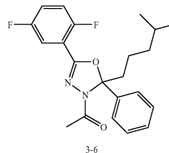
3-[3-acetyl-5-(2,5-difluorophenyl)-2-phenyl-2,3-dihydro-1,3,4-oxadiazol-2-yl]-N,N-dimethylpropan-1-amine (3-6)
