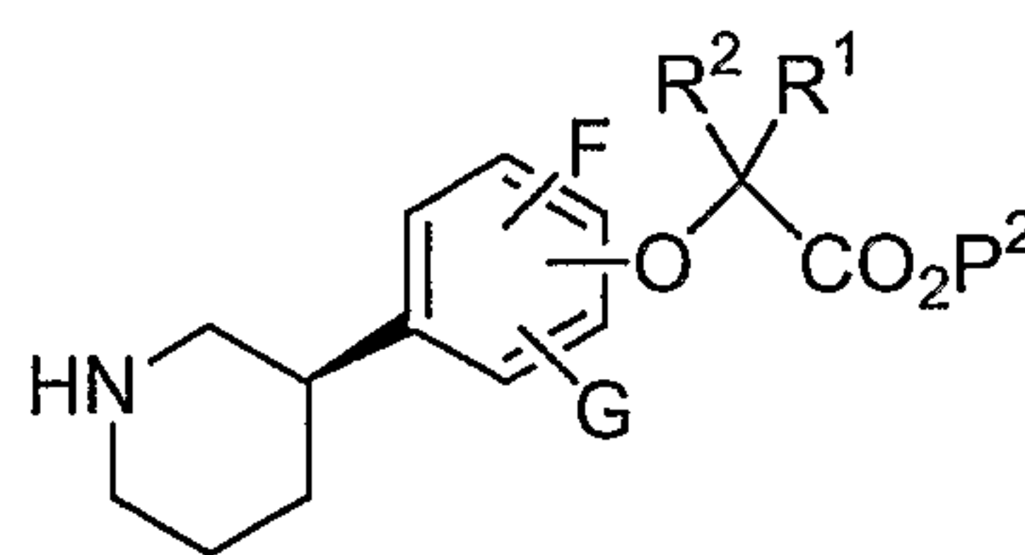
III (R)
