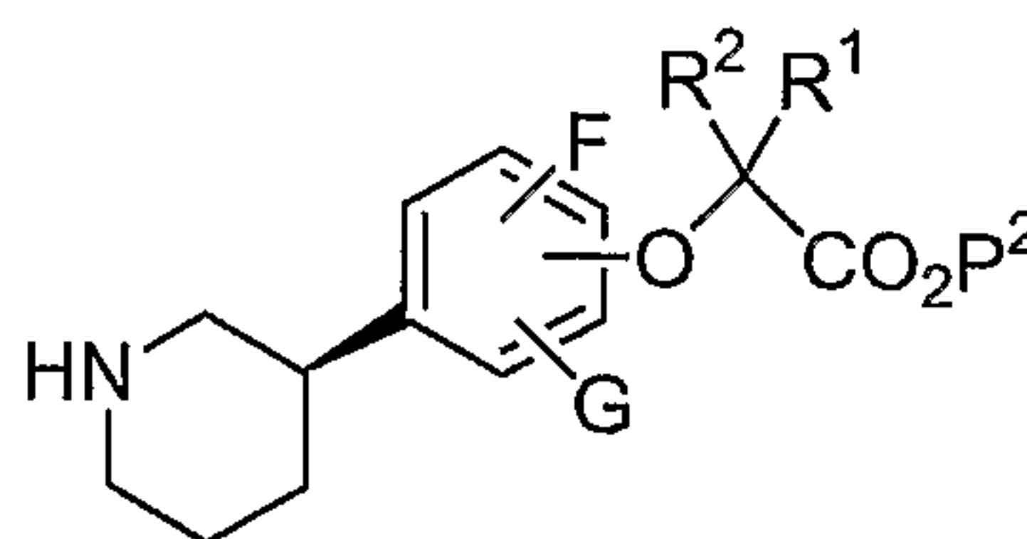
III (R)
