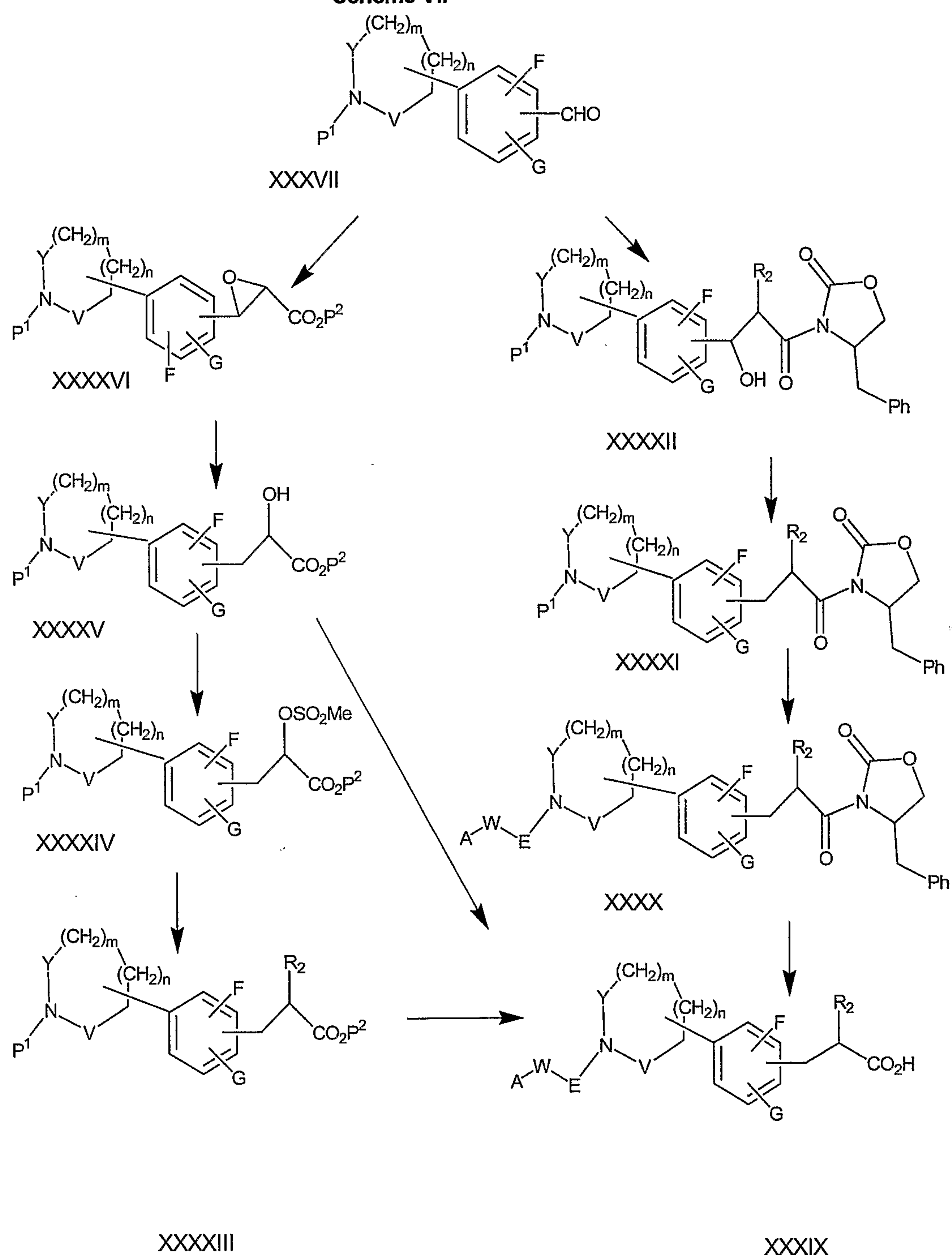
Scheme VII
