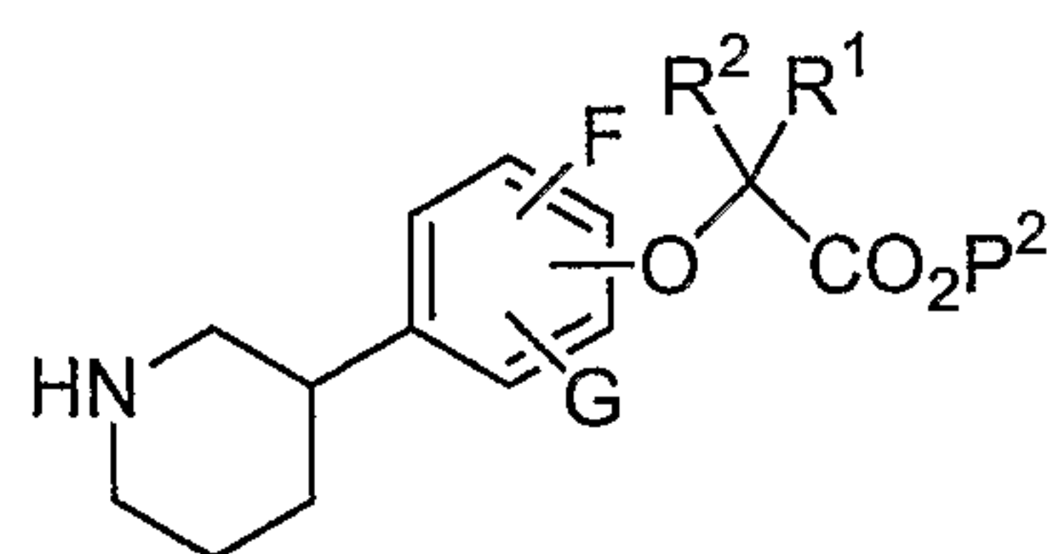
III
