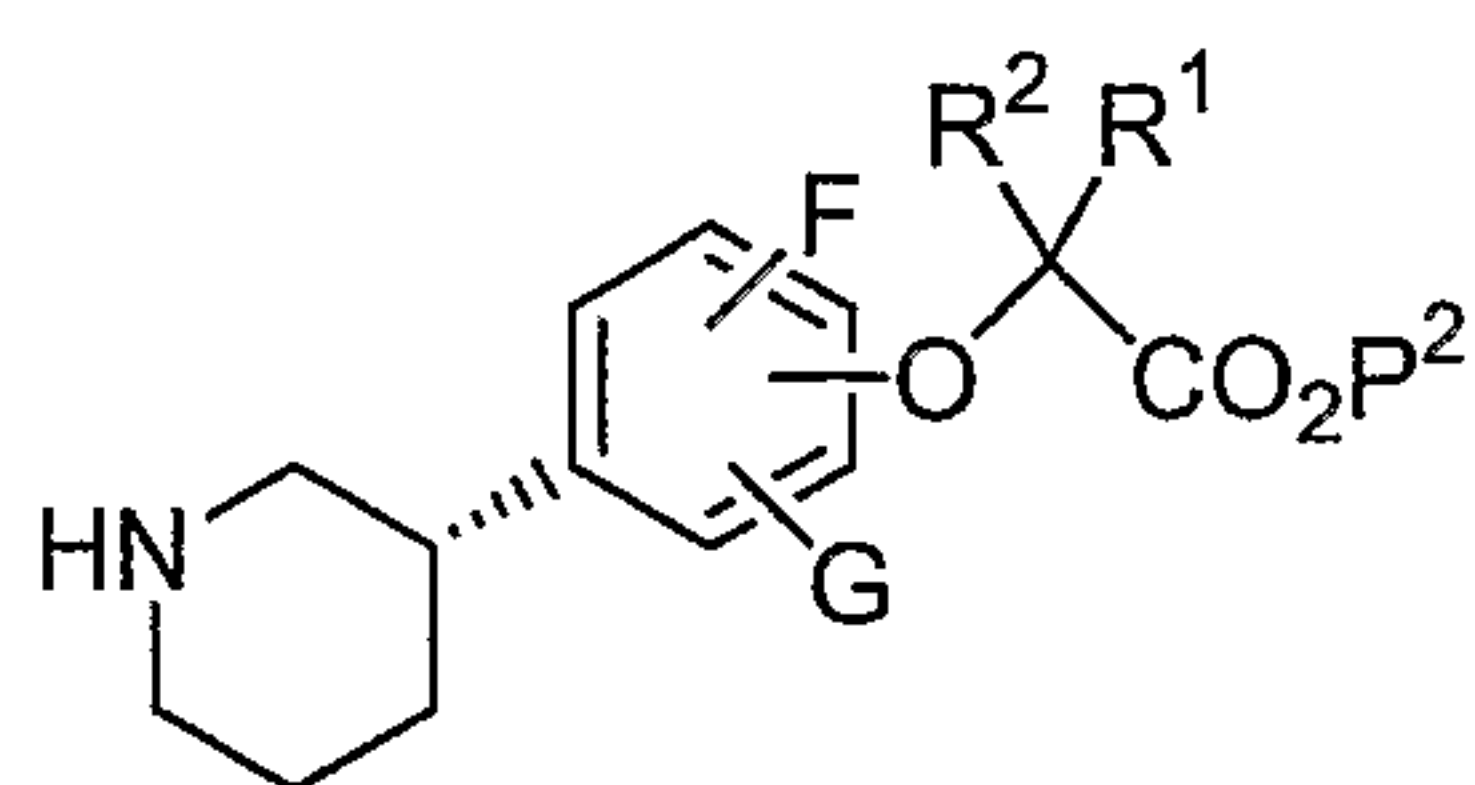
III (S)
