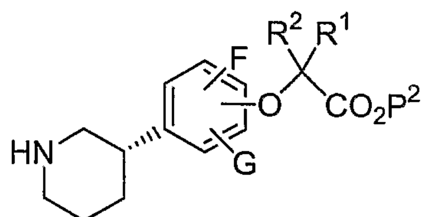
III (S)
