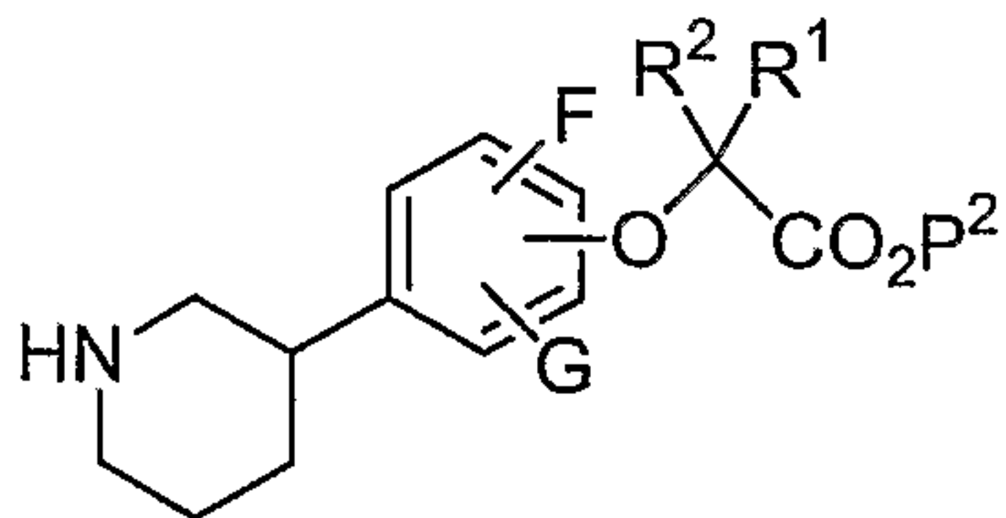
III
