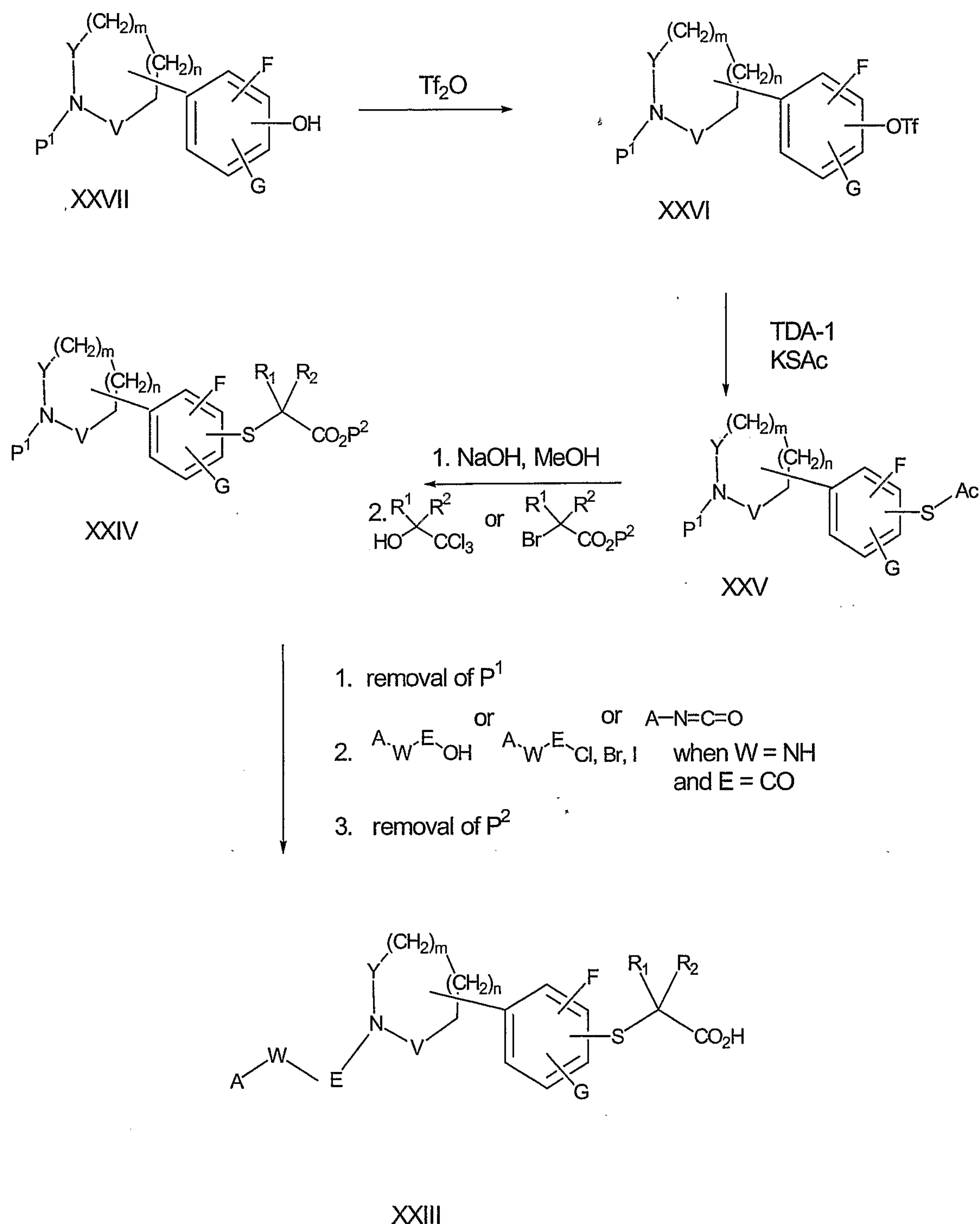
Scheme IV
