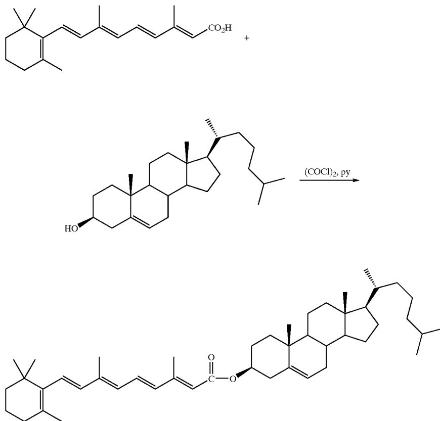
(SCHEME 4)
