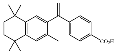
SR11247
