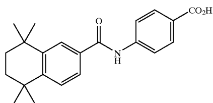
Am580
