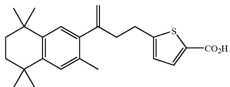
SR11251
