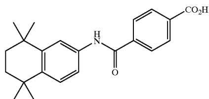
Am80
