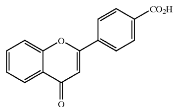
Flavone-4'-carboxylic acids
