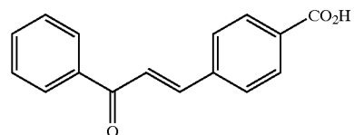
Chalcone-4-carboxylic acids
