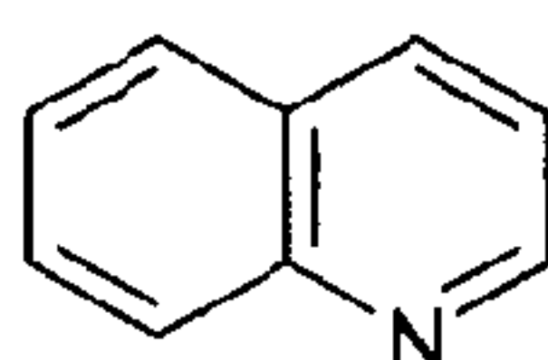
quinoline
