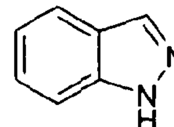
indazole
