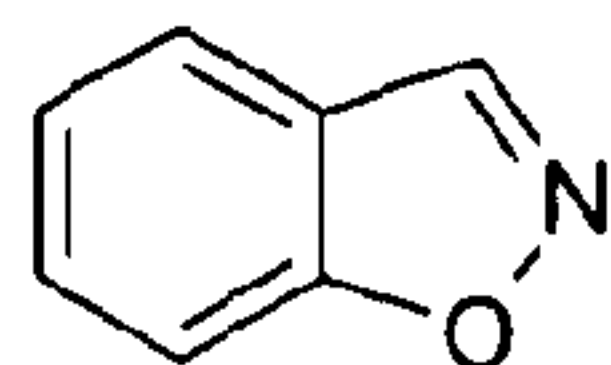
benzoxazole
