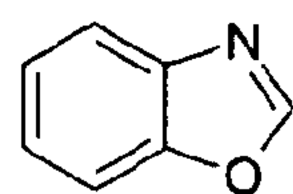
benzoxazole
