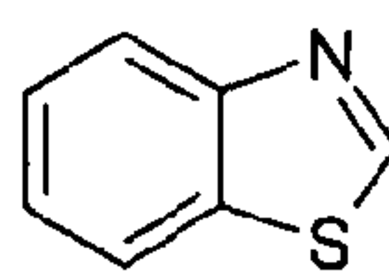
benzothiazole
