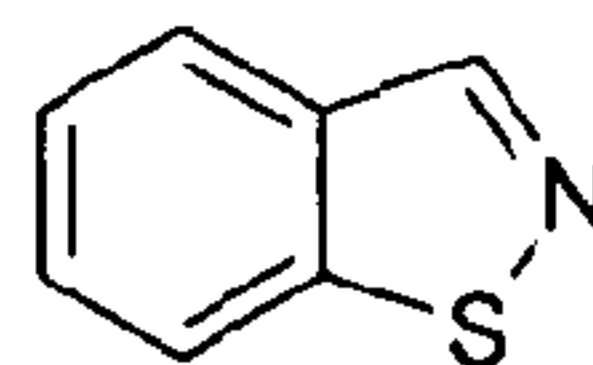
benzoisothiazole
