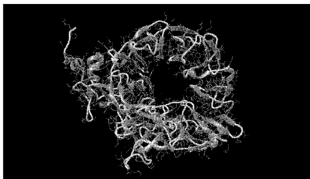
FIGURE 1: Sortilin.
