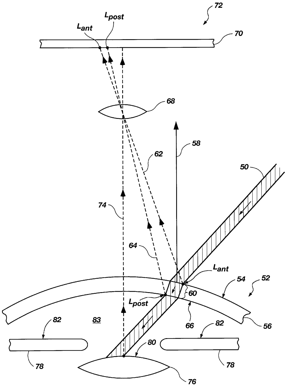
Fig. 3 (PRIOR ART)
