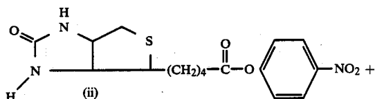
Biotin-p-nitrophenyl ester
