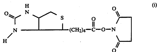
Biotin-N-hydroxysuccinimide
