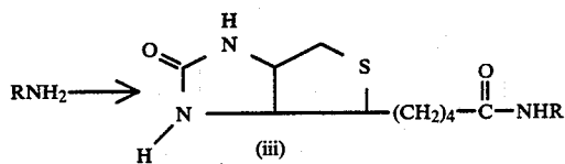
Biotin-p-nitrophenyl ester
