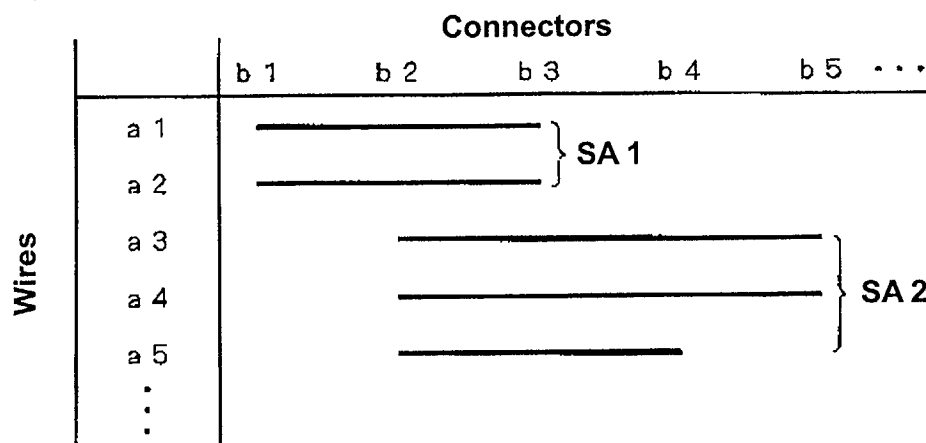
FIG. 50 PRIOR ART
