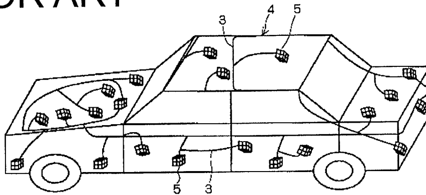
FIG. 15 PRIOR ART
