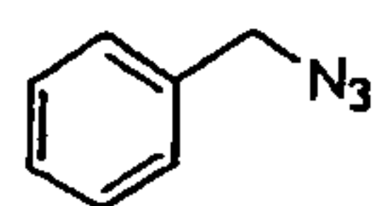
Benzyl azide
