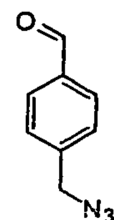
Aldehyde azide
