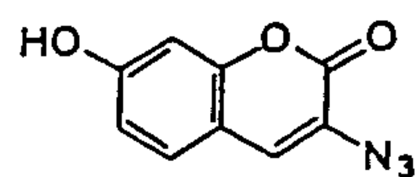
Coumarin azide
