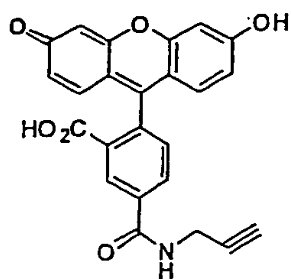
Fluorescein alkyne
