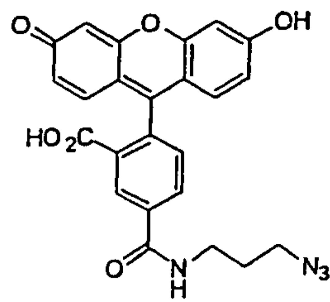
Fluorescein azide
