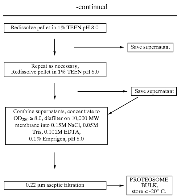
Manufacture of Proteosome Bulk Material: FLOWCHART 1A
