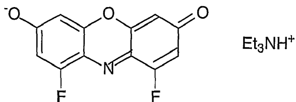
Compound 15
