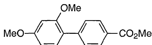
Compound 23
