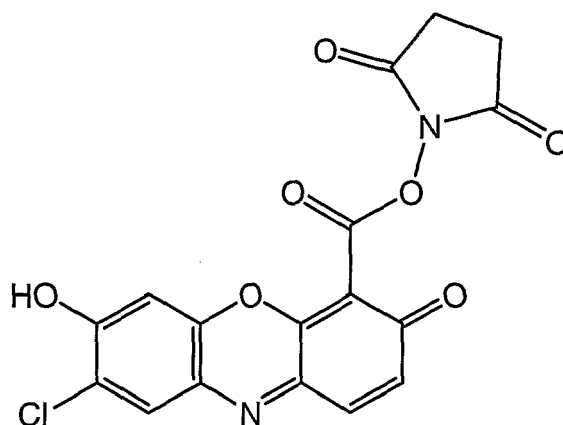
Compound 21
