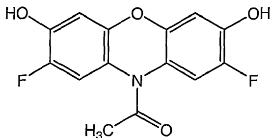
Compound 4
