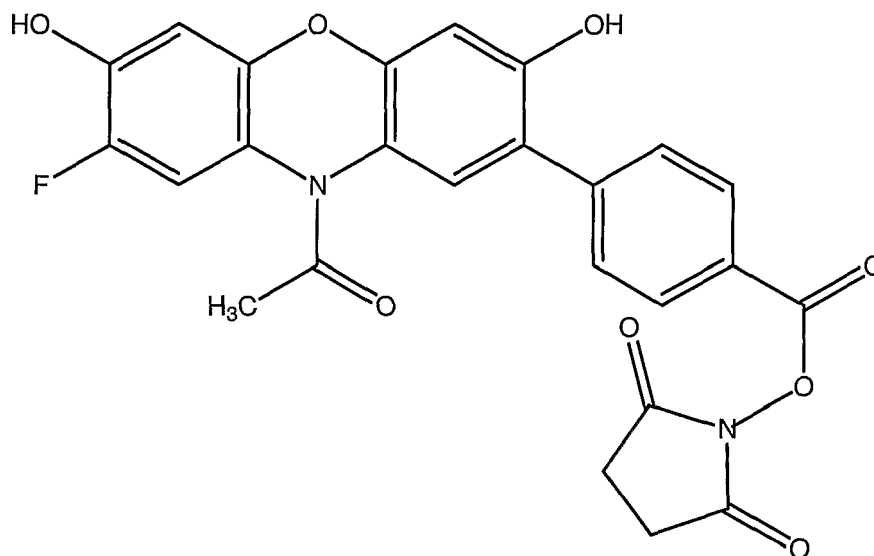
Compound 28
