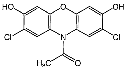
Compound 19
