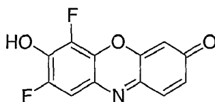
Compound 5
