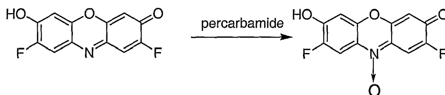
Compound 32
