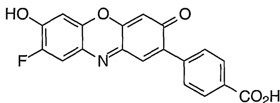
Compound 25
