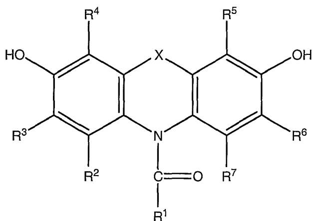
Formula II(b)
