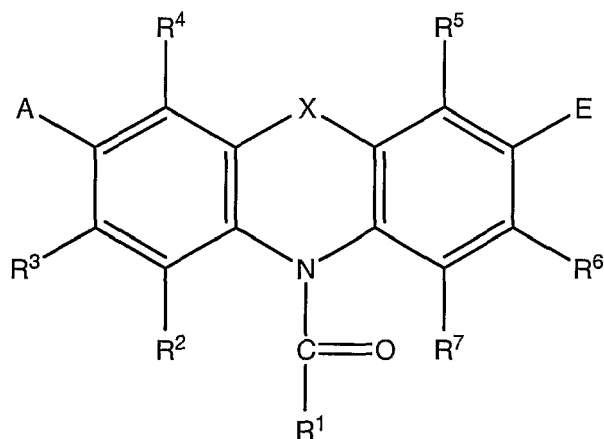
Formula II(a)
