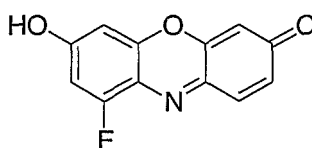
Compound 8
