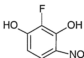
.....Compound 10
