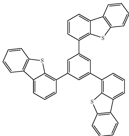
(i) DBT3P-II
