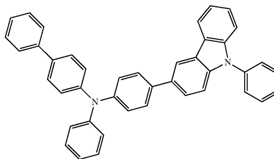
(iv) PCBA1BP
