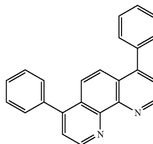
(xi) Bphen
