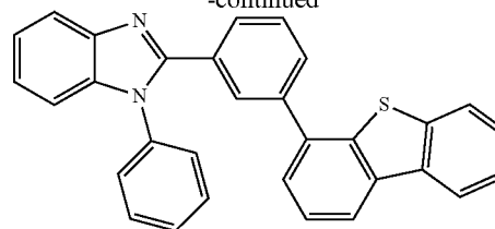
(x) mDBTBIIm-II
