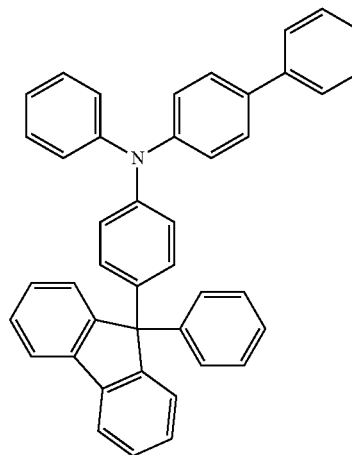
(ii) BPAFLP
