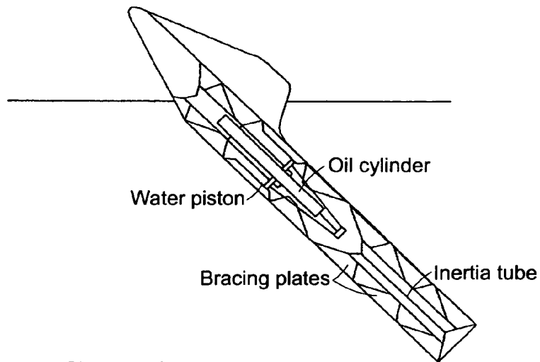
Sloped IPS Buoy — Free Floating (Prior Art)
