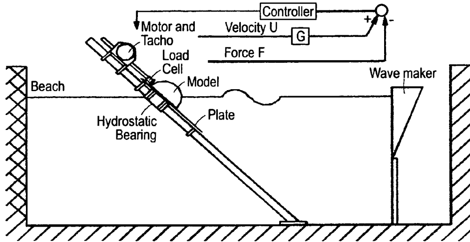
Sloped IPS Buoy — Fixed Position (Prior Art)
